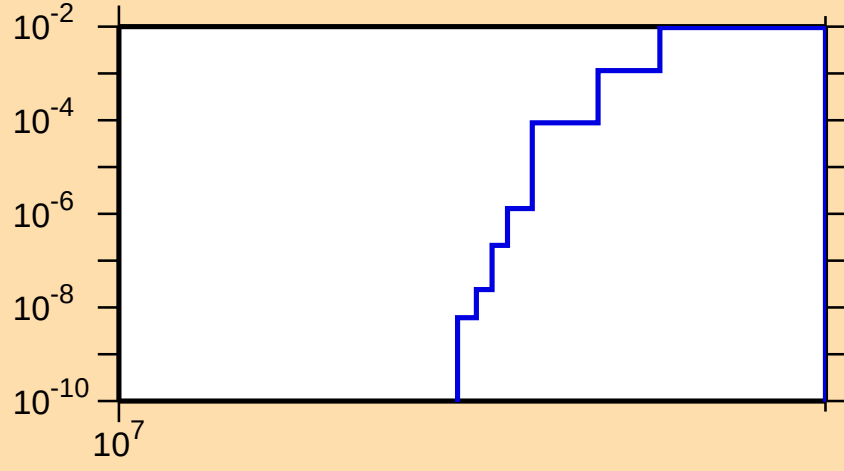
\sigma vs. E for ^{100}\text{Rh}(n,2np)
