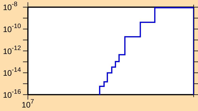
\sigma vs. E for ^{100}\text{Rh}(\text{mt } 45)
