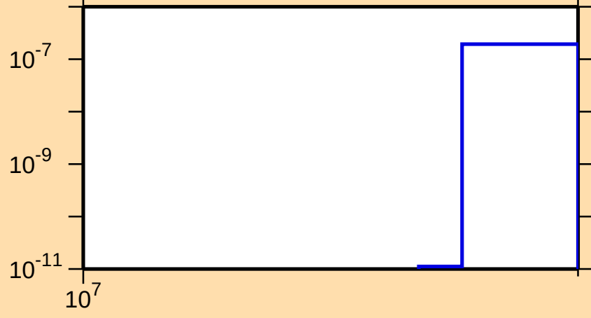
\sigma vs. E for ^{100}\text{Rh}(n,nt)
