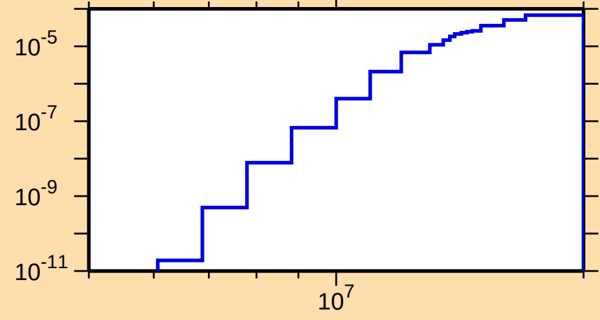
\sigma vs. E for ^{100}\text{Rh}(n,p\alpha)
