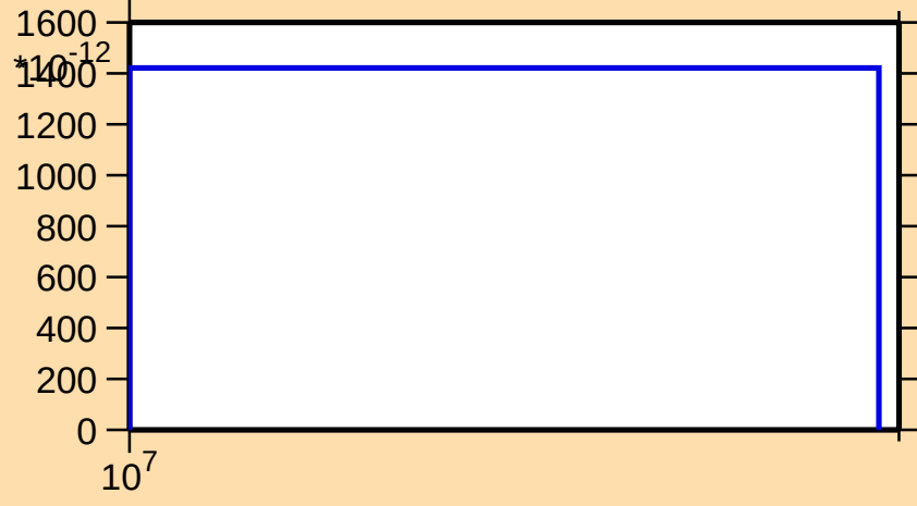
\sigma vs. E for ^{100}\text{Rh}(n,\text{nt})
