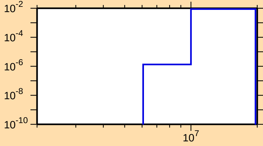
\sigma vs. E for ^{100}\text{Rh}(n,\alpha)
