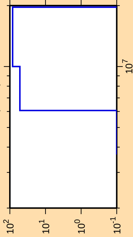
\Delta\sigma/\sigma vs. E for ^{100}\text{Rh}(n,\alpha)
