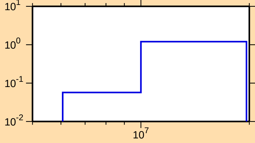
\sigma vs. E for ^{100}\text{Rh}(n,2n)
