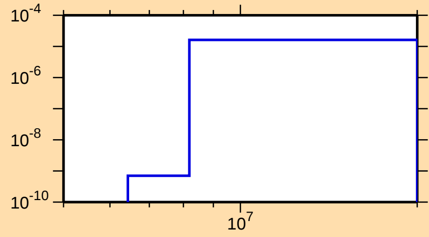
\sigma vs. E for ^{100}\text{Rh}(n,p\alpha)
