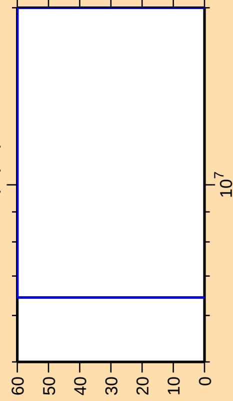
\Delta\sigma/\sigma vs. E for ^{100}\text{Rh}(n,p\alpha)
