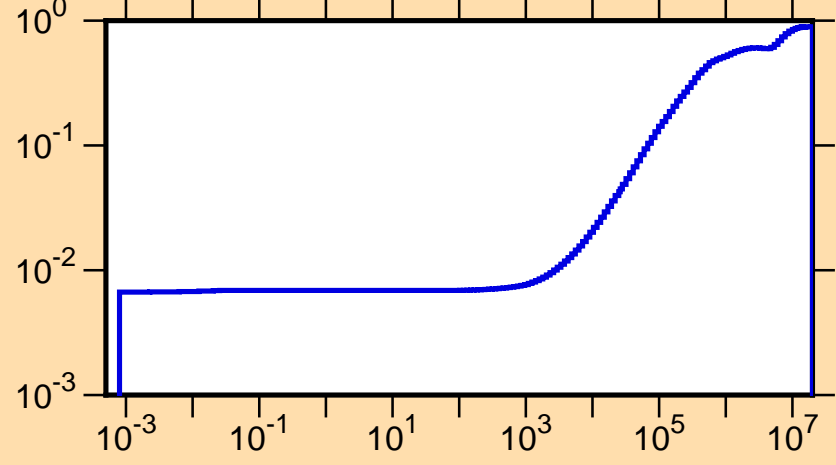
\mu vs. E for ^{101}\text{Rh}(\text{mt251})
