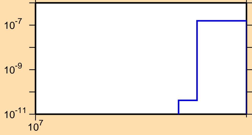
\sigma vs. E for ^{101}\text{Rh}(n,nt)
