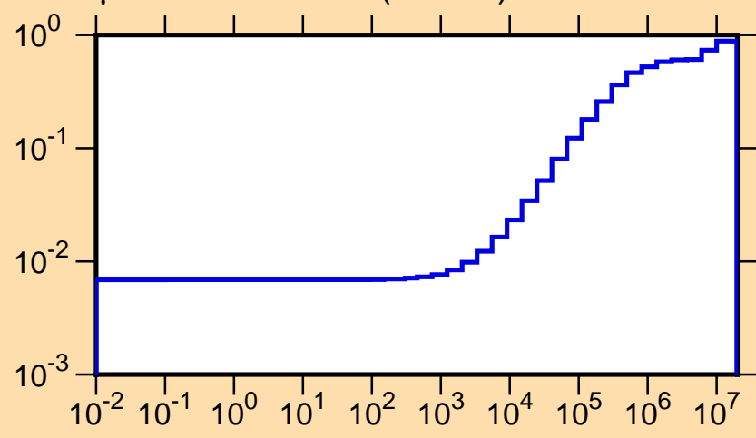
\mu vs. E for ^{101}\text{Rh}(\text{mt251})
