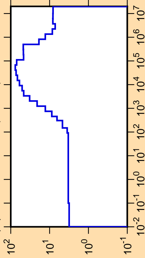
\Delta\mu/\mu vs. E for ^{101}\text{Rh}(\text{mt251})
