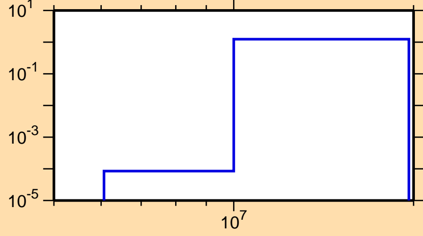
\sigma vs. E for ^{101}\text{Rh}(n,2n)
