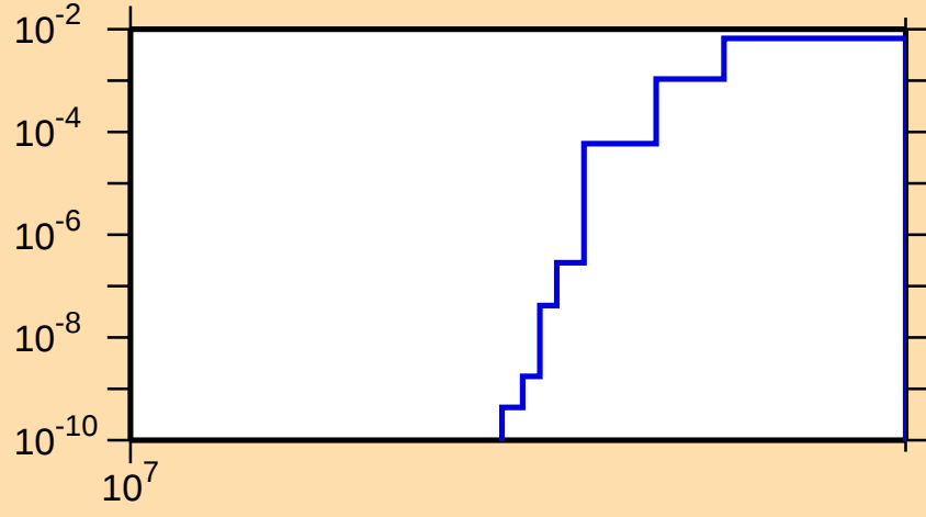
\sigma vs. E for ^{102}\text{Rh}(n,2np)
