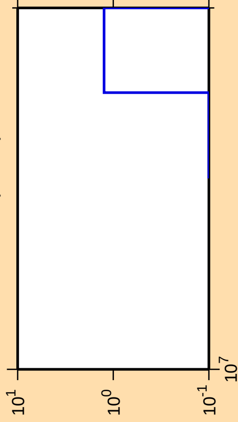
\Delta\sigma/\sigma vs. E for ^{102}\text{Rh}(\text{mt } 34)
