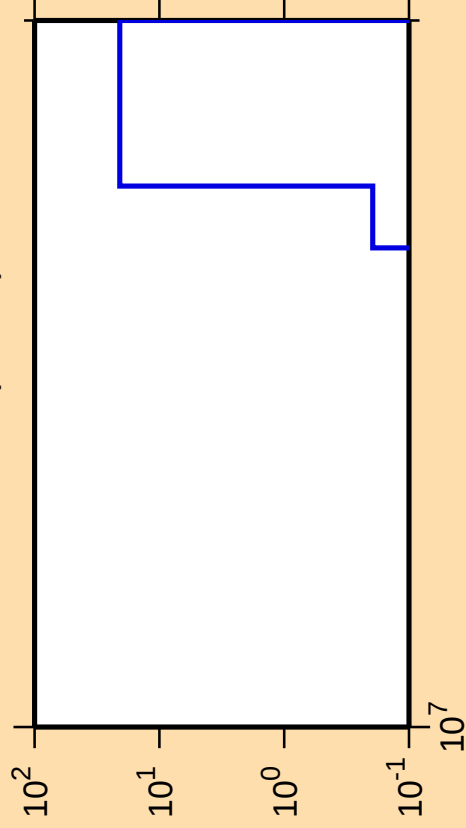
\Delta\sigma/\sigma vs. E for ^{102}\text{Rh}(\text{mt } 45)
