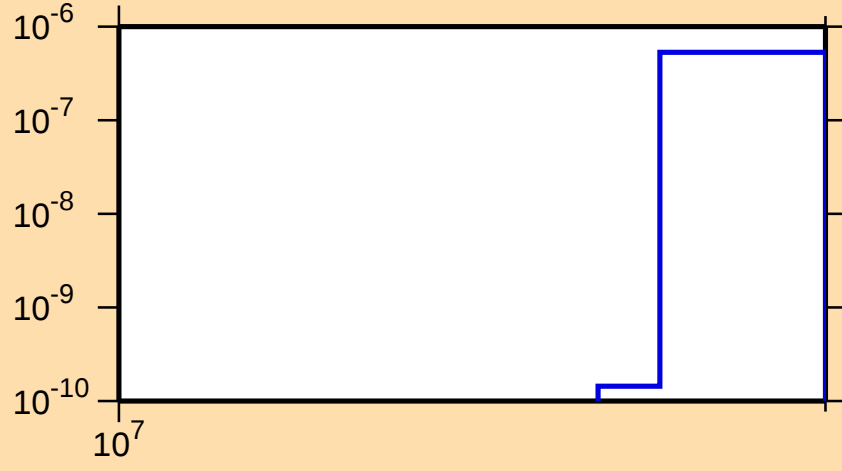
\sigma vs. E for ^{102}\text{Rh}(n,\text{nt})
