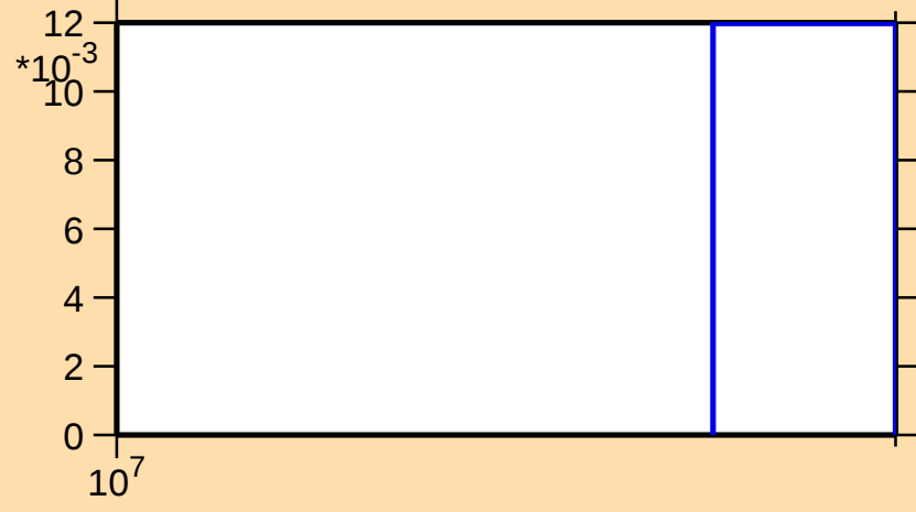
\sigma vs. E for ^{102}\text{Rh}(n,3n)
