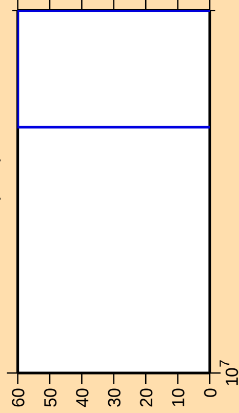
\Delta\sigma/\sigma vs. E for ^{102}\text{Rh}(n,\text{nt})
