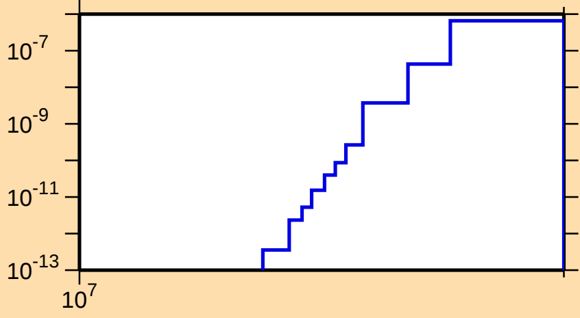
\sigma vs. E for ^{102}\text{Rh}(n,\text{He3})
