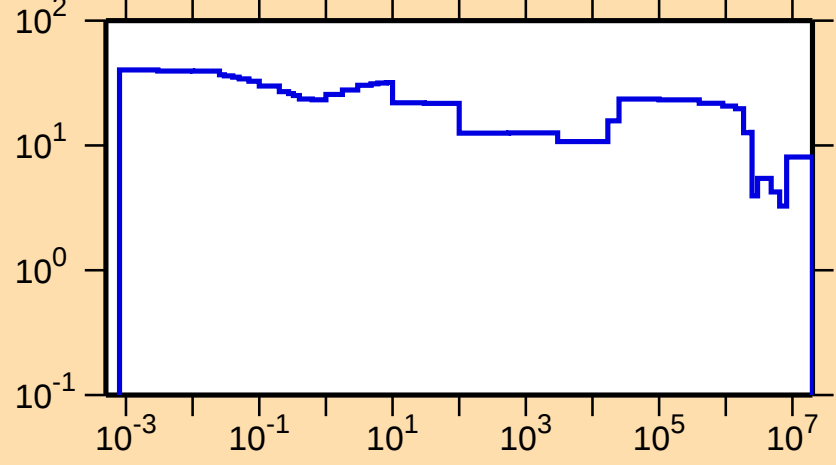
\Delta\sigma/\sigma vs. E for ^{102}\text{Rh}(n,\text{tot.})
