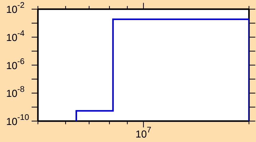
\sigma vs. E for ^{102}\text{Rh}(n,\alpha)
