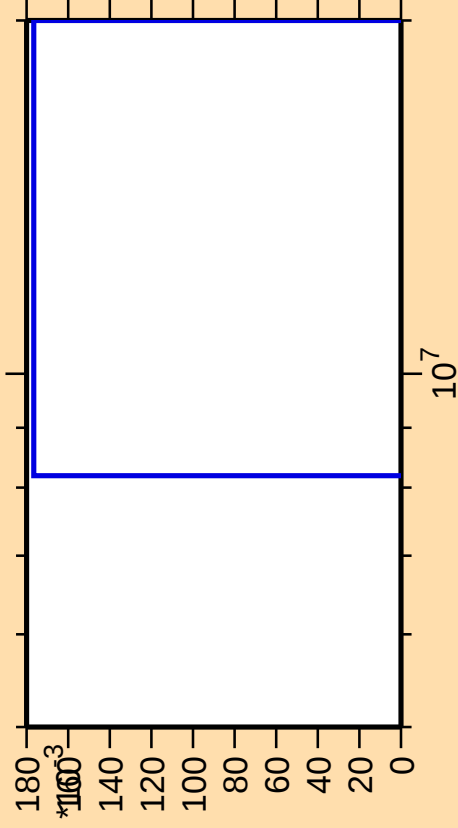
\Delta\sigma/\sigma vs. E for ^{102}\text{Rh}(\text{mt } 45)
