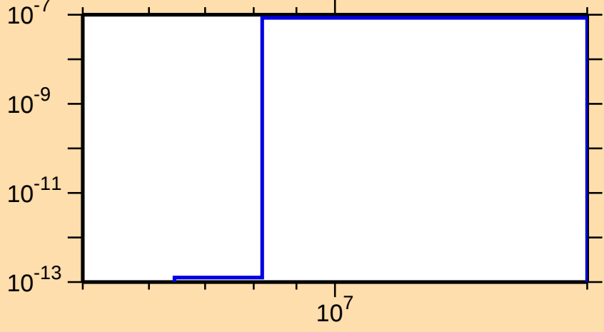
\sigma vs. E for ^{102}\text{Rh}(n,p\alpha)
