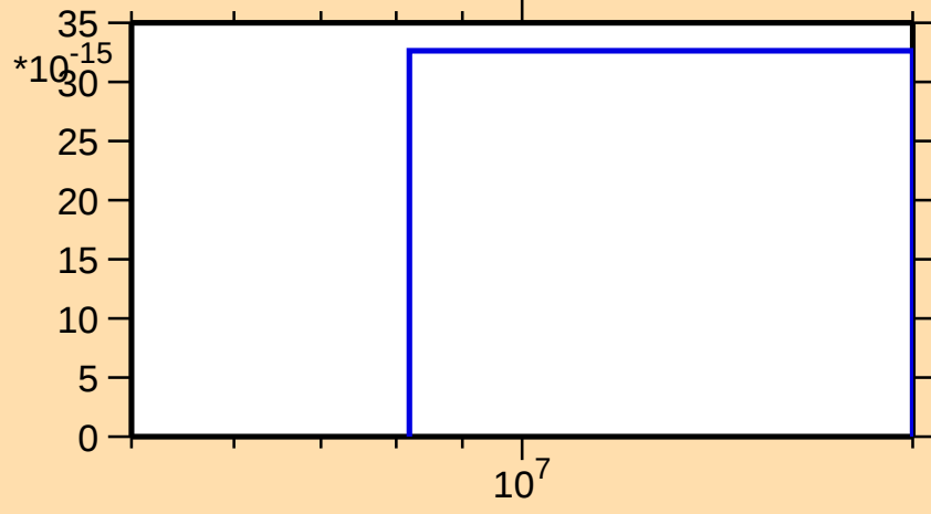
\sigma vs. E for ^{102}\text{Rh}(\text{mt } 45)
