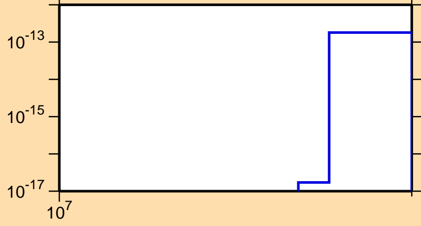
\sigma vs. E for ^{102}\text{Rh}(\text{mt } 34)
