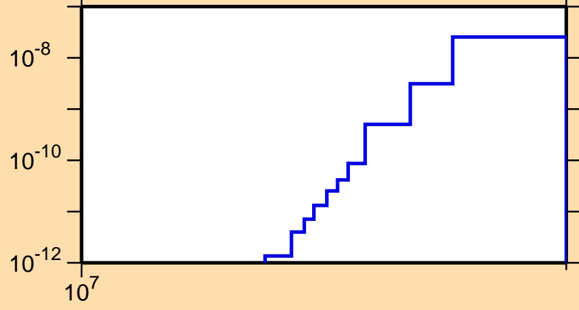
\sigma vs. E for ^{103}\text{Rh}(n,p\alpha)
