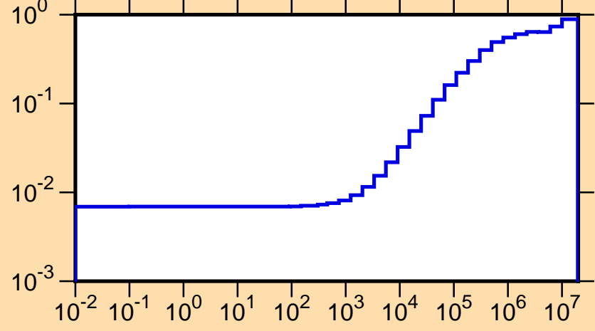
\mu vs. E for ^{103}\text{Rh}(\text{mt251})
