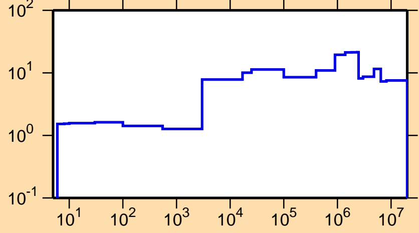
\Delta\sigma/\sigma vs. E for ^{103}\text{Rh}(n,\text{el.})
