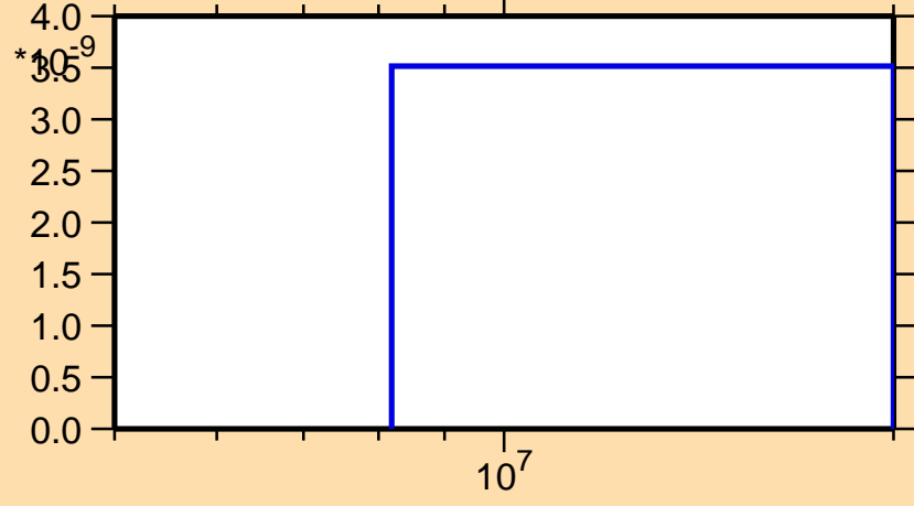
\sigma vs. E for ^{103}\text{Rh}(n,nt)
