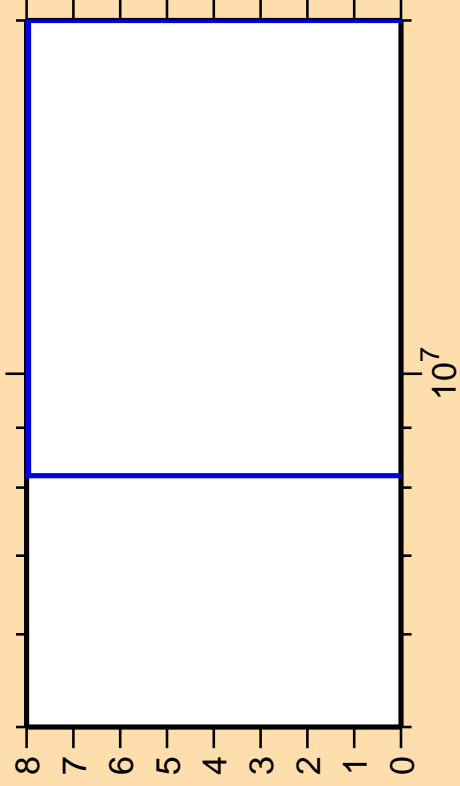
\Delta\sigma/\sigma vs. E for ^{103}\text{Rh}(n,2n)
