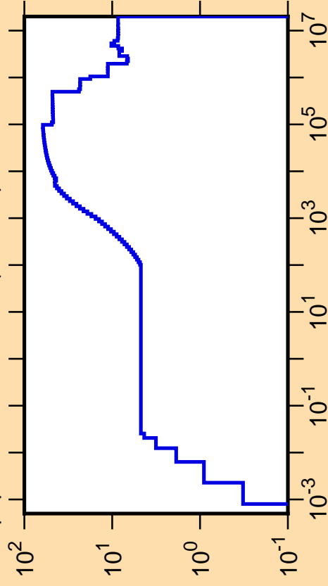
\Delta\mu/\mu vs. E for ^{105}\text{Rh}(\text{mt251})
