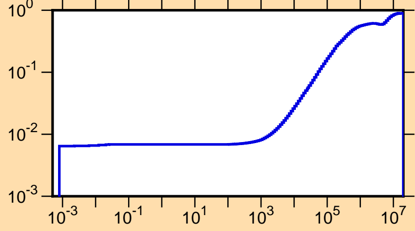
\mu vs. E for ^{105}\text{Rh}(\text{mt251})
