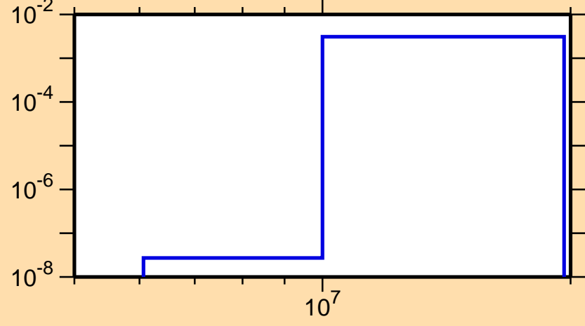
\sigma vs. E for ^{105}\text{Rh}(n,np)
