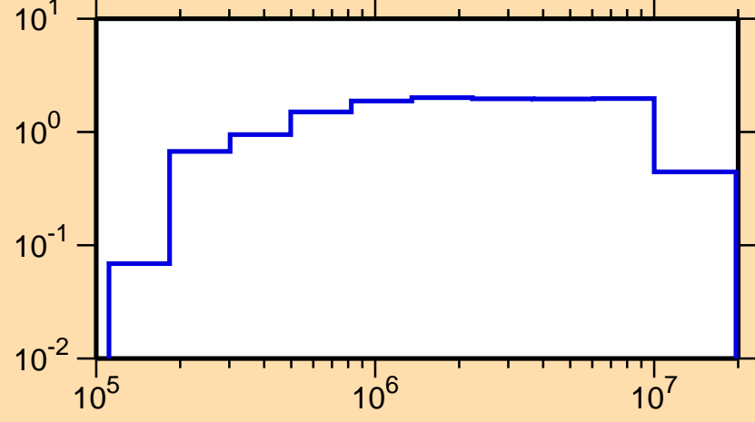
\sigma vs. E for ^{105}\text{Rh}(n,\text{inel.})
