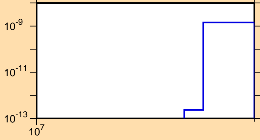
\sigma vs. E for ^{105}\text{Rh}(n,2n\alpha)
