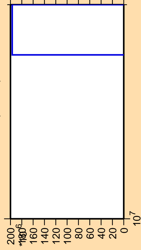
\Delta\sigma/\sigma vs. E for ^{105}\text{Rh}(n,3n\alpha)
