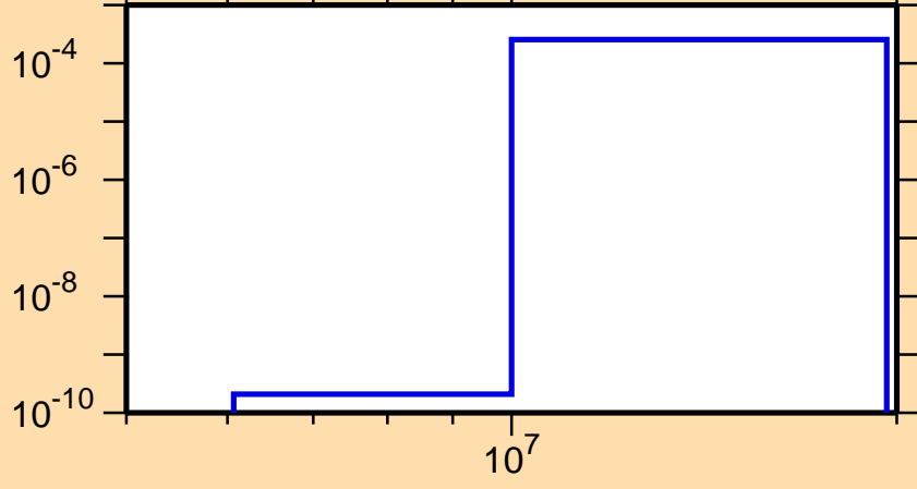
\sigma vs. E for ^{105}\text{Rh}(n,\alpha)
