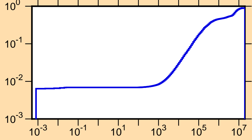
\mu vs. E for ^{106}\text{Rh}(\text{mt251})
