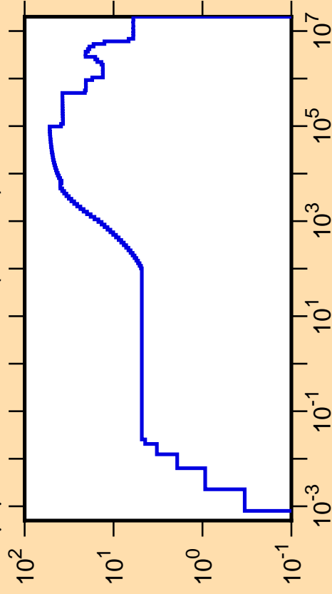
\Delta\mu/\mu vs. E for ^{106}\text{Rh}(\text{mt251})
