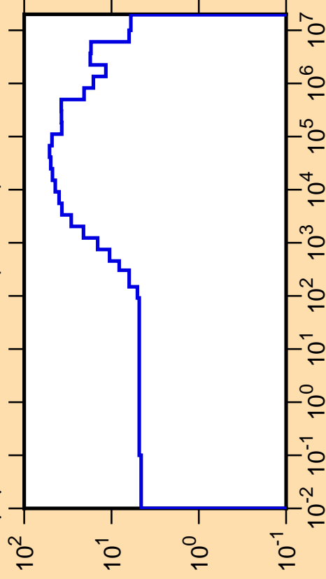
\Delta\mu/\mu vs. E for ^{106}\text{Rh}(\text{mt251})
