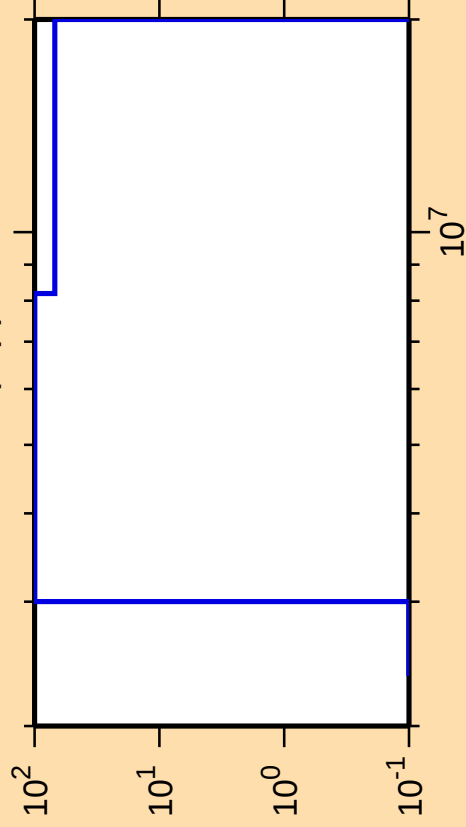
\Delta\sigma/\sigma vs. E for ^{107}\text{Rh}(n,p)
