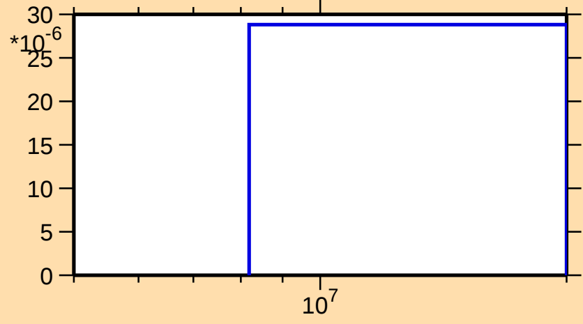
\sigma vs. E for ^{107}\text{Rh}(n,\alpha)
