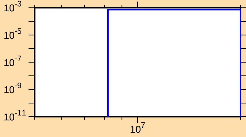
\sigma vs. E for ^{107}\text{Rh}(n,np)
