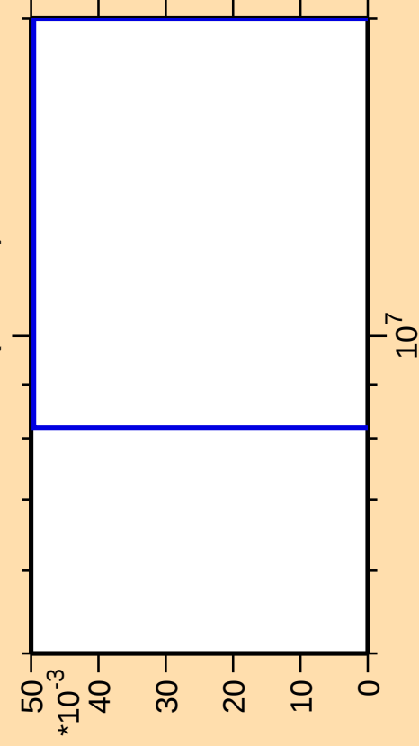
\Delta\sigma/\sigma vs. E for ^{107}\text{Rh}(n,\text{He3})
