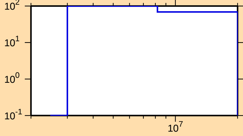
\Delta\sigma/\sigma vs. E for ^{107}\text{Rh}(n,p)
