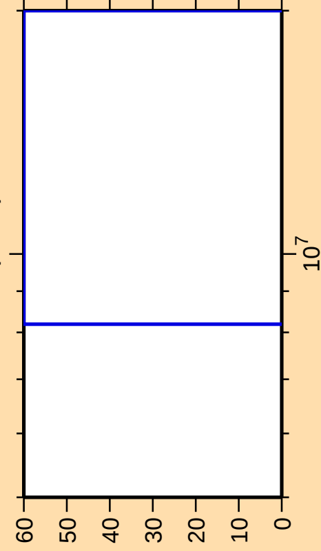
\Delta\sigma/\sigma vs. E for ^{107}\text{Rh}(n,\alpha)
