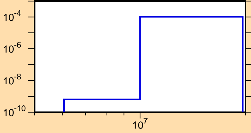
\sigma vs. E for ^{108}\text{Rh}(n,t)
