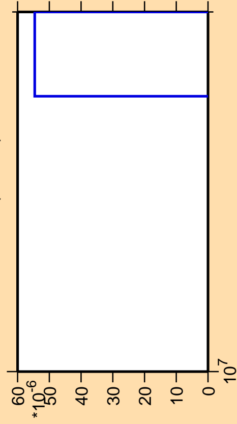
\Delta\sigma/\sigma vs. E for ^{108}\text{Rh}(n,3n\alpha)
