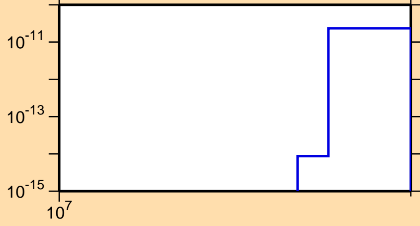
\sigma vs. E for ^{108}\text{Rh}(n,\text{He3})
