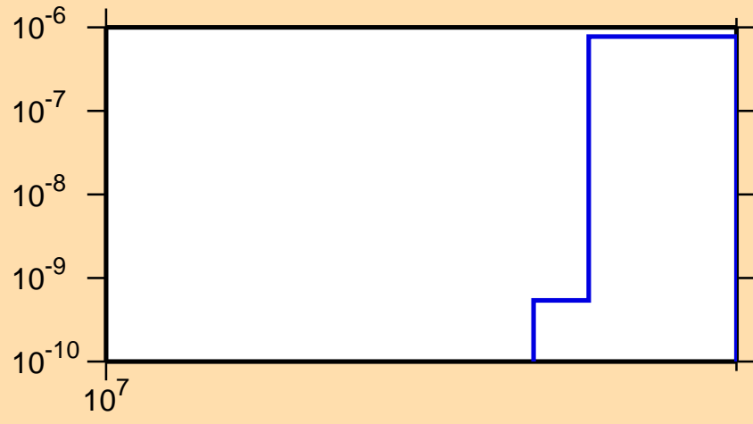
\sigma vs. E for ^{108}\text{Rh}(n,\text{nt})
