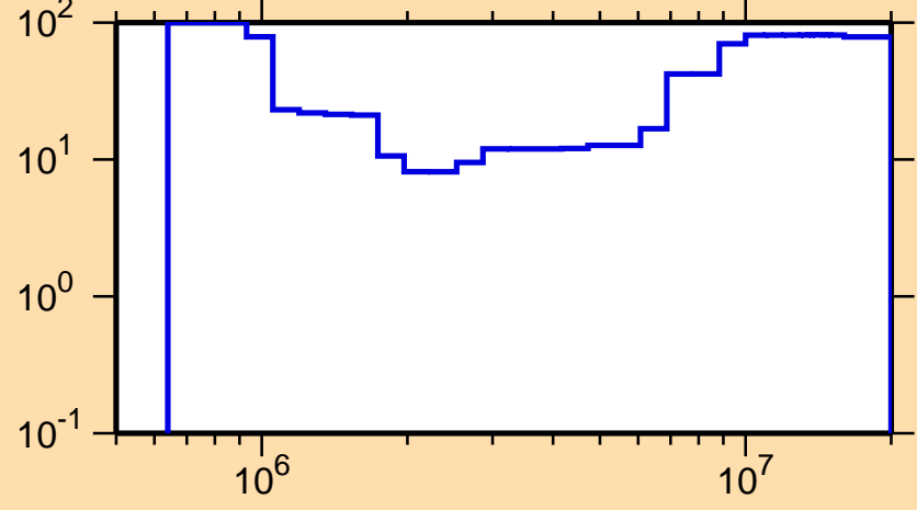
\Delta\sigma/\sigma vs. E for ^{108}\text{Rh}(n,n\text{cont.})
