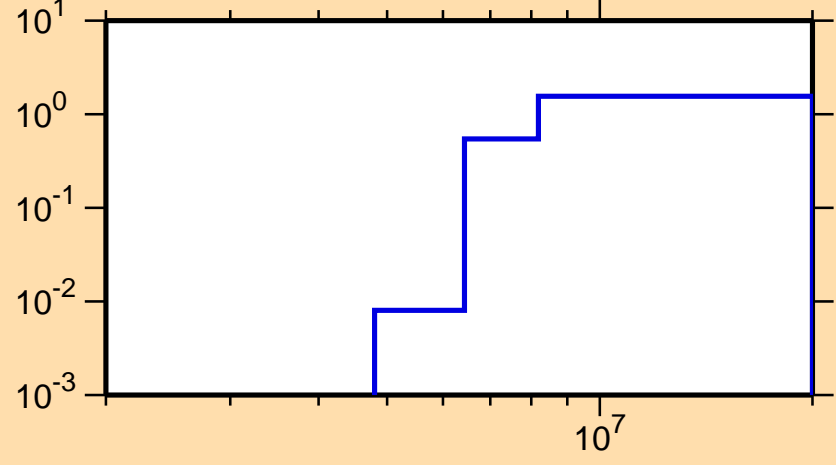
\sigma vs. E for ^{108}\text{Rh}(n,2n)
