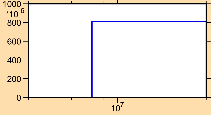
\sigma vs. E for ^{108}\text{Rh}(n,np)
