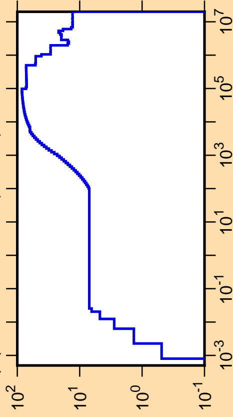
\Delta\mu/\mu vs. E for ^{109}\text{Rh}(\text{mt251})
