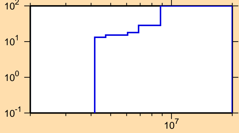
\Delta\sigma/\sigma vs. E for ^{109}\text{Rh}(n,ncont.)
