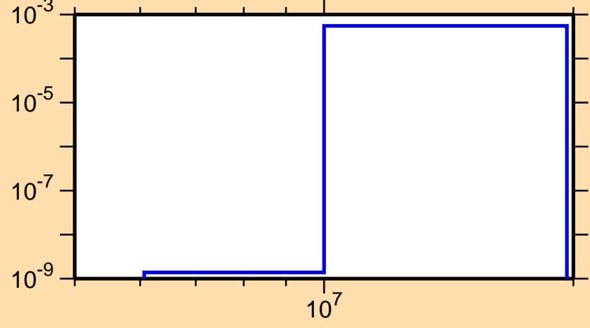
\sigma vs. E for ^{109}\text{Rh}(n,d)
