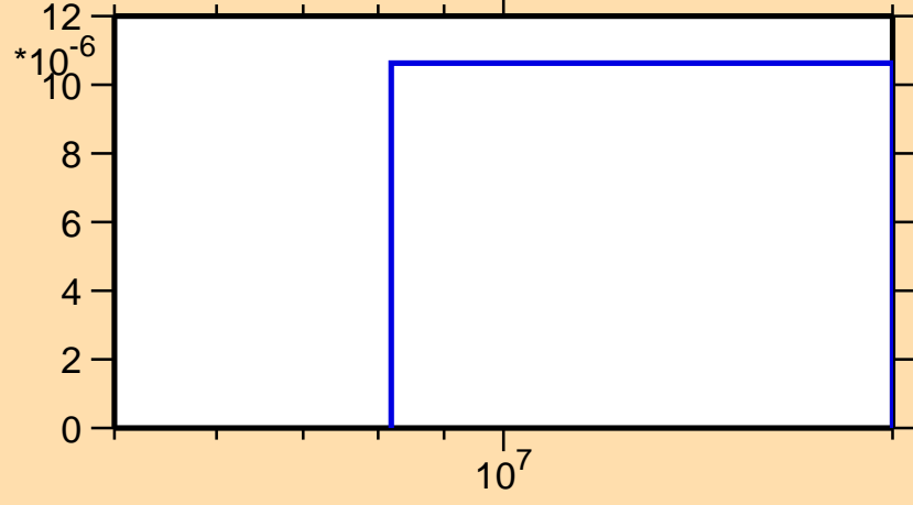
\sigma vs. E for ^{109}\text{Rh}(n,t)
