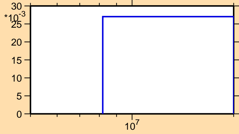
\sigma vs. E for ^{109}\text{Rh}(n,3n)
