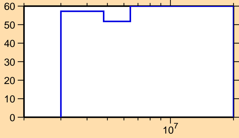
\Delta\sigma/\sigma vs. E for ^{109}\text{Rh}(n,n_1)
