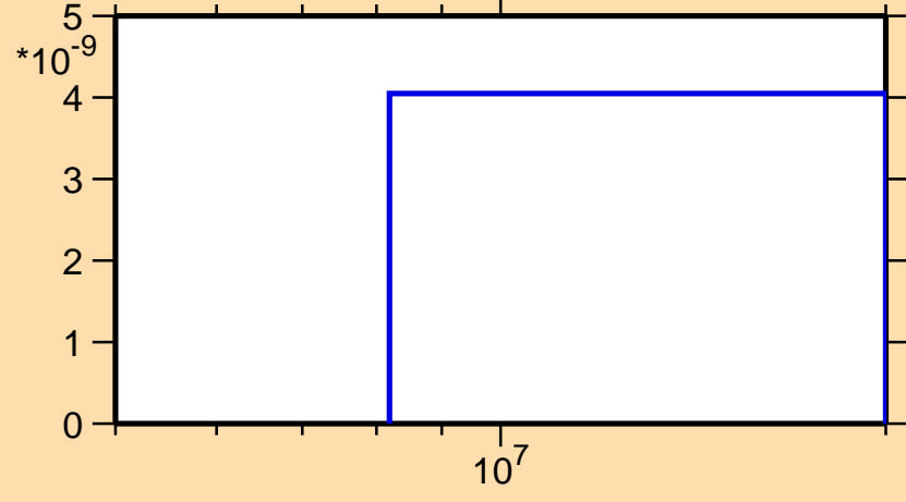
\sigma vs. E for ^{109}\text{Rh}(n,nt)
