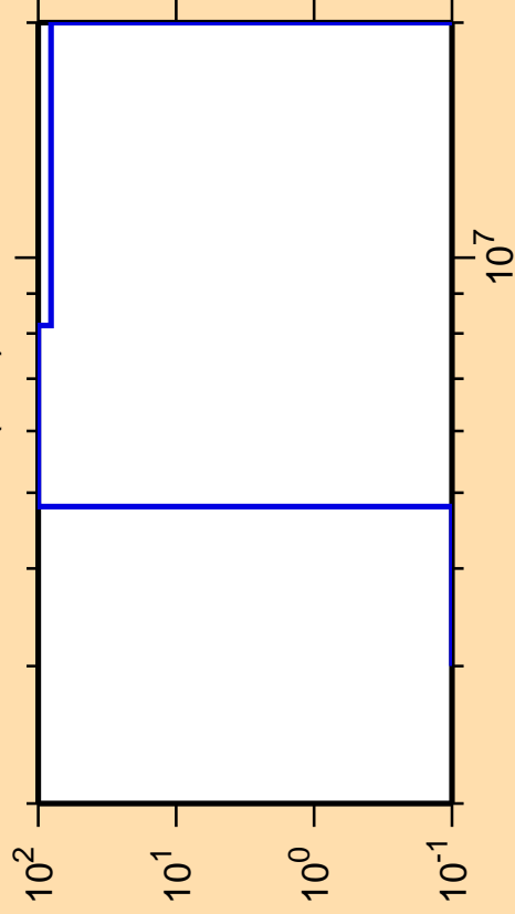
\Delta\sigma/\sigma vs. E for ^{109}\text{Rh}(n,\alpha)
