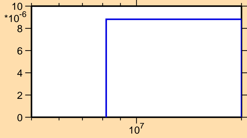
\sigma vs. E for ^{109}\text{Rh}(n,\alpha)
