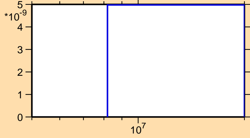
\sigma vs. E for ^{109}\text{Rh}(n,\text{nd})
