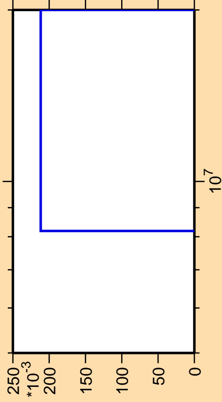
\Delta\sigma/\sigma vs. E for ^{109}\text{Rh}(n,2n\alpha)
