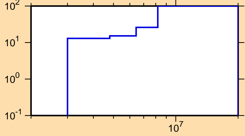
\Delta\sigma/\sigma vs. E for ^{109}\text{Rh}(n,n\text{cont.})
