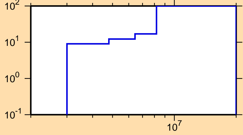
\Delta\sigma/\sigma vs. E for ^{109}\text{Rh}(n,\text{inel.})
