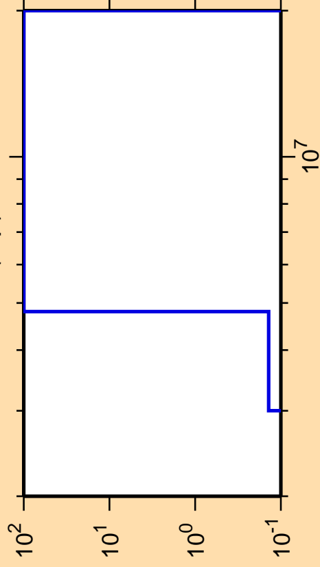
\Delta\sigma/\sigma vs. E for ^{109}\text{Rh}(n,p)
