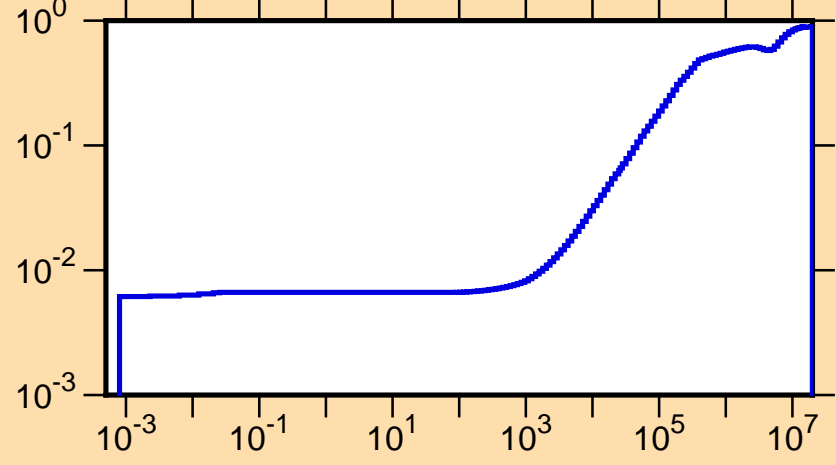
\mu vs. E for ^{110}\text{Rh}(\text{mt251})
