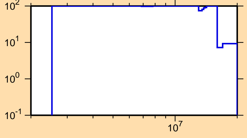
\Delta\sigma/\sigma vs. E for ^{110}\text{Rh}(n,n_1)
