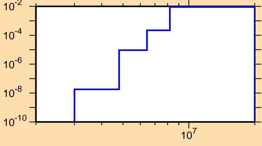
\sigma vs. E for ^{110}\text{Rh}(n,p)
