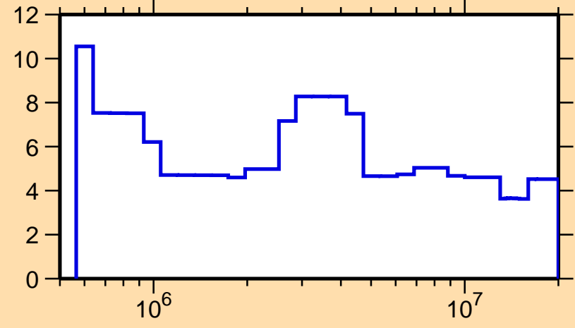
\Delta\sigma/\sigma vs. E for ^{110}\text{Rh}(n,n\text{nonel.})
