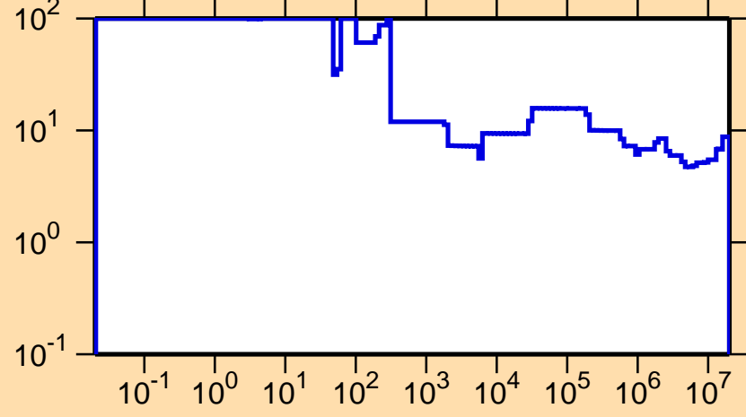
\Delta\sigma/\sigma vs. E for ^{110}\text{Rh}(n,\text{el.})
