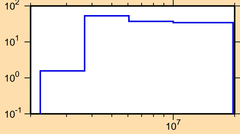
\Delta\sigma/\sigma vs. E for ^{110}\text{Rh}(n,p)
