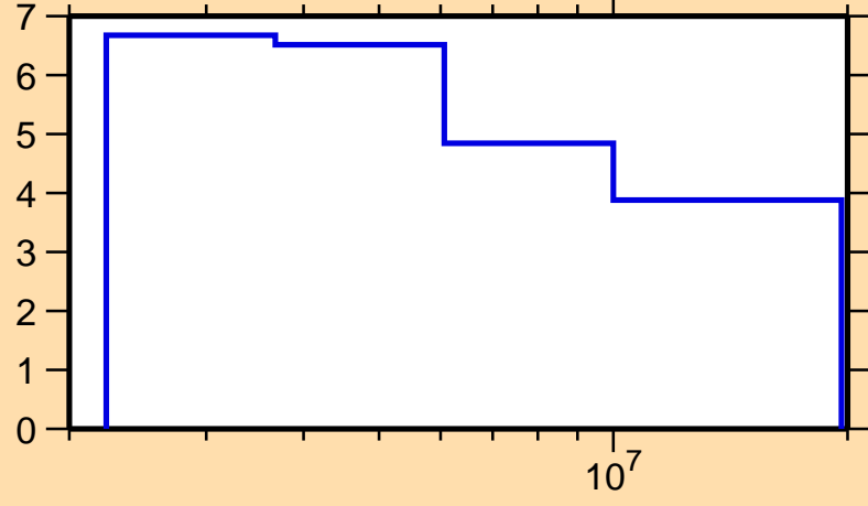
\Delta\sigma/\sigma vs. E for ^{110}\text{Rh}(n,\text{nonel.})
