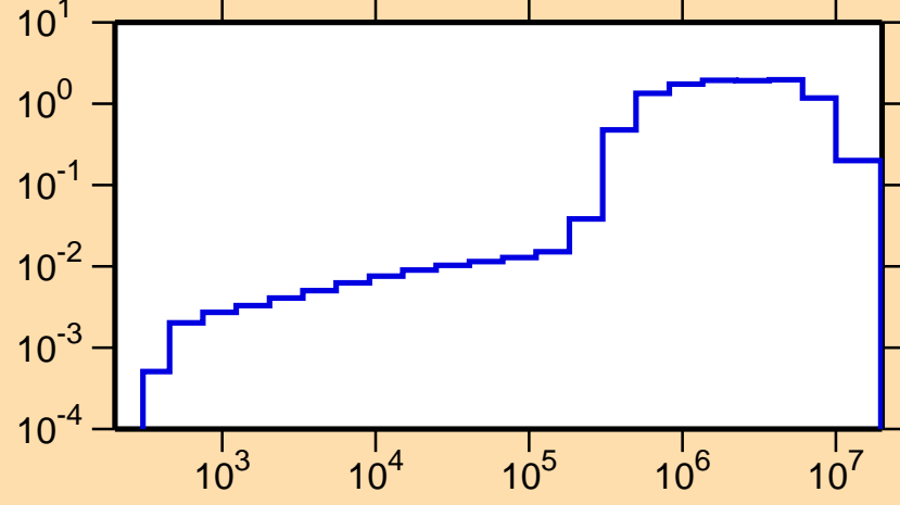
\sigma vs. E for ^{110}\text{Rh}(n,\text{inel.})
