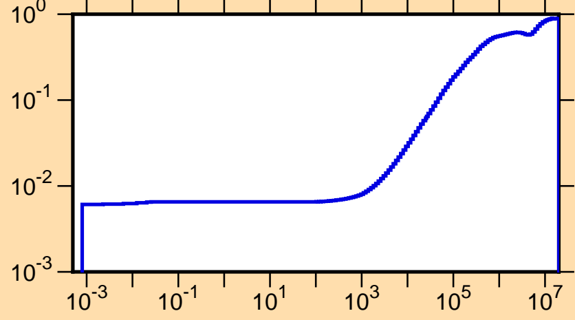
\mu vs. E for ^{111}\text{Rh}(\text{mt251})
