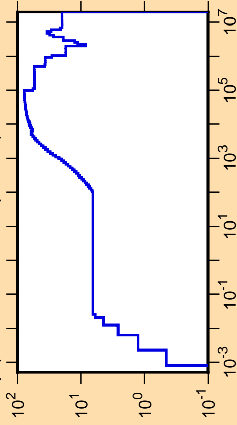
\Delta\mu/\mu vs. E for ^{111}\text{Rh}(\text{mt251})
