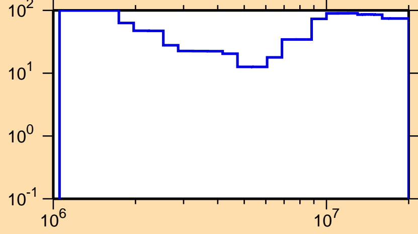
\Delta\sigma/\sigma vs. E for ^{111}\text{Rh}(n,n\text{cont.})
