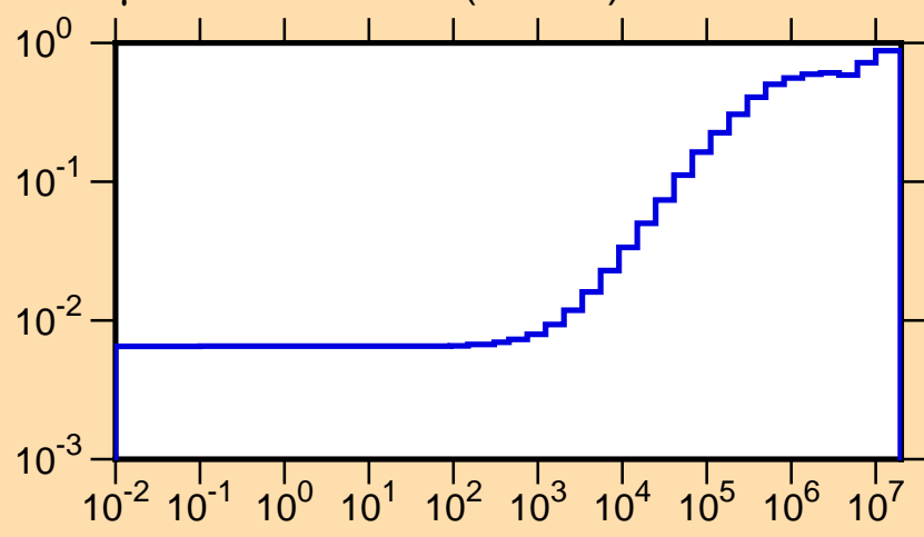
\mu vs. E for ^{111}\text{Rh}(\text{mt251})
