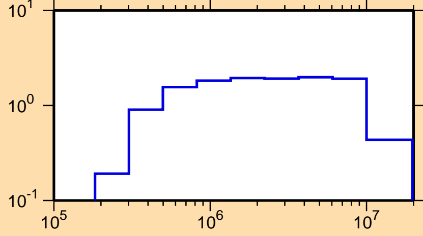
\sigma vs. E for ^{111}\text{Rh}(n,\text{inel.})
