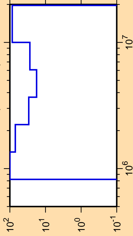
\Delta\sigma/\sigma vs. E for ^{111}\text{Rh}(n,\text{ncont.})
