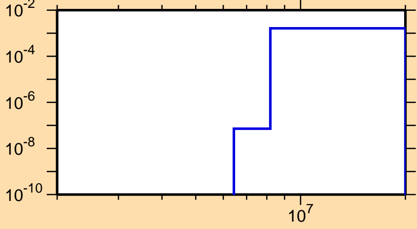
\sigma vs. E for ^{111}\text{Rh}(n,p)
