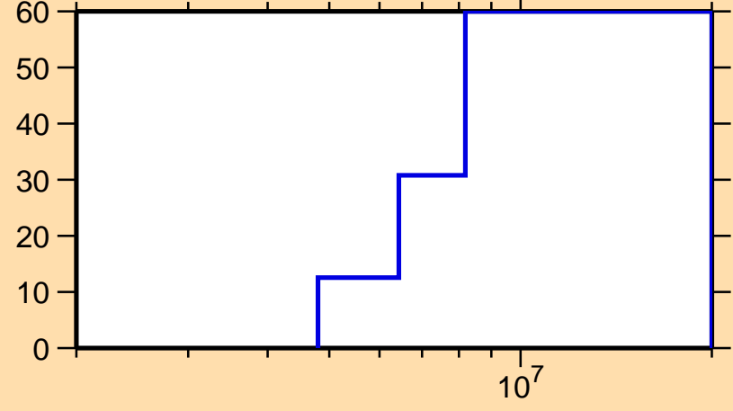
\Delta\sigma/\sigma vs. E for ^{111}\text{Rh}(n,ncont.)
