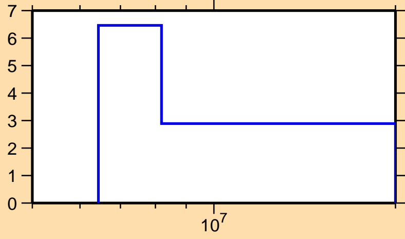
\Delta\sigma/\sigma vs. E for ^{111}\text{Rh}(n,\text{nonel.})
