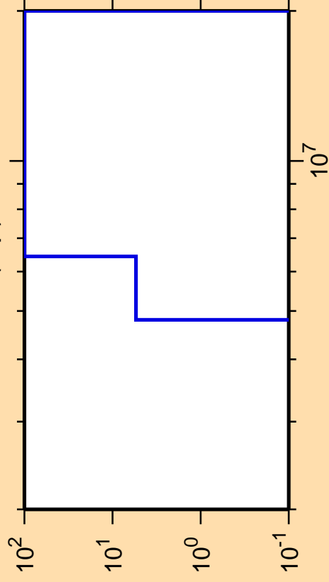
\Delta\sigma/\sigma vs. E for ^{111}\text{Rh}(n,p)
