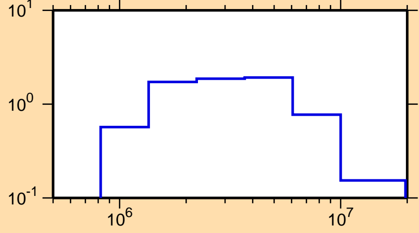
\sigma vs. E for ^{114}\text{Rh}(n,n\text{cont.})
