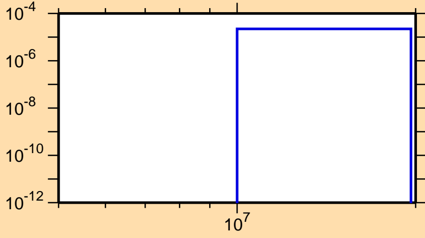
\sigma vs. E for ^{114}\text{Rh}(n,t)
