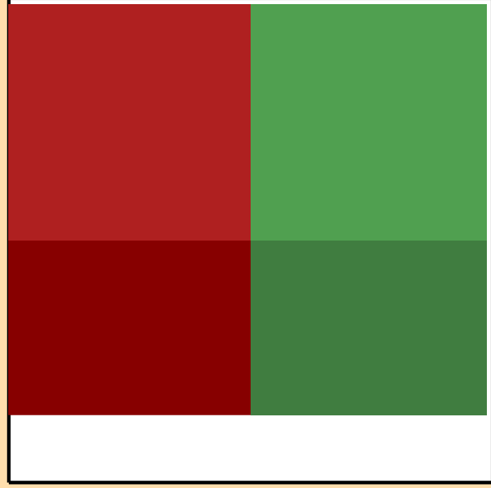
\Delta\sigma/\sigma vs. E for ^{114}\text{Rh}(n,n_1)
