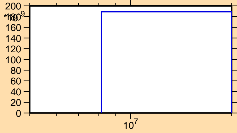
\sigma vs. E for ^{114}\text{Rh}(n,\alpha)
