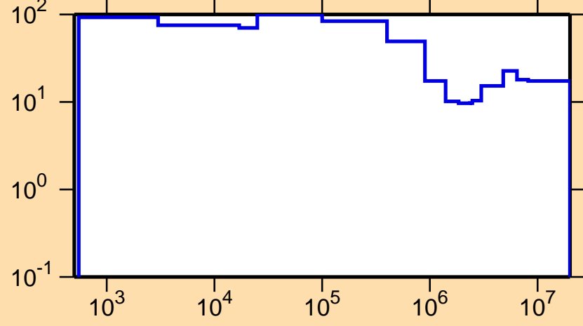
\Delta\sigma/\sigma vs. E for ^{114}\text{Rh}(n,\text{nonel.})
