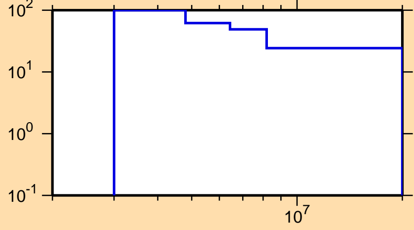
\Delta\sigma/\sigma vs. E for ^{114}\text{Rh}(n,2n)
