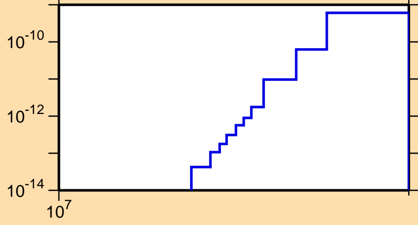
\sigma vs. E for ^{201}\text{Rn}(\text{mt } 34)
