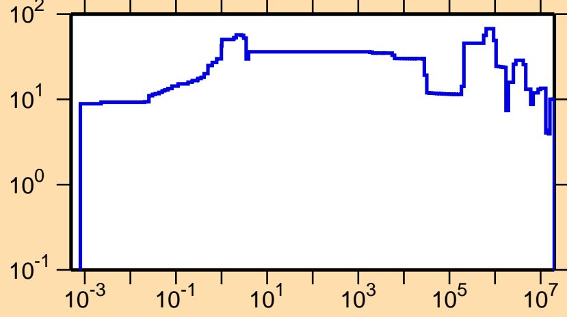
\Delta\sigma/\sigma vs. E for ^{201}\text{Rn}(n,\text{tot.})
