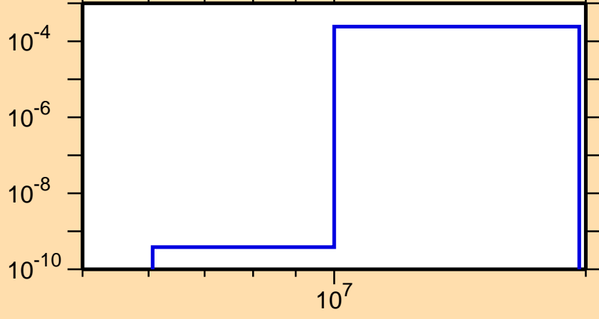
\sigma vs. E for ^{201}\text{Rn}(n,t)
