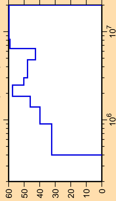
\Delta\sigma/\sigma vs. E for ^{201}\text{Rn}(n,\text{inel.})
