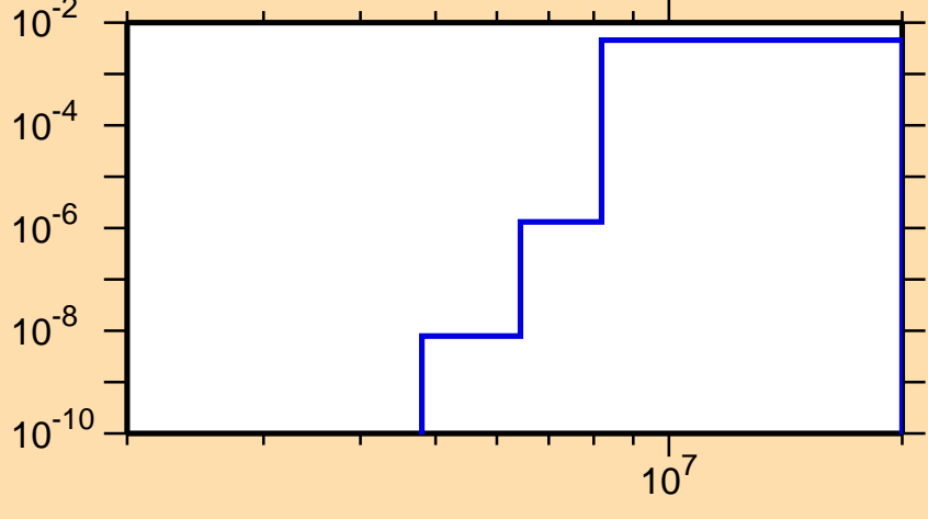
\sigma vs. E for ^{201}\text{Rn}(n,d)
