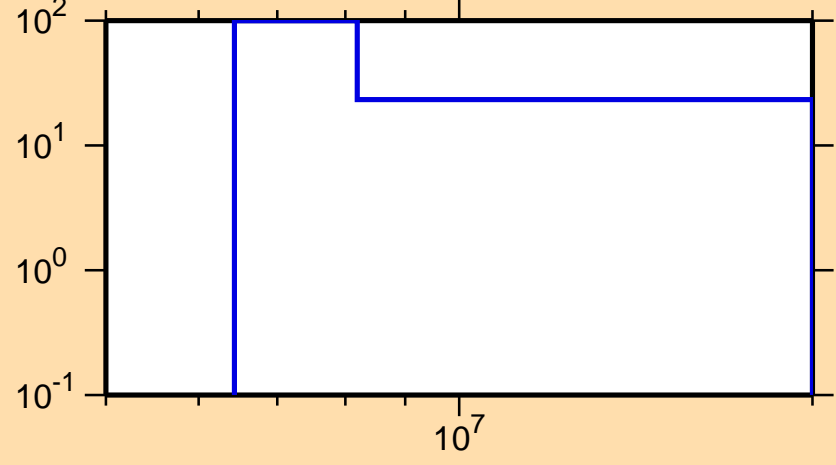
\Delta\sigma/\sigma vs. E for ^{201}\text{Rn}(n,2n)
