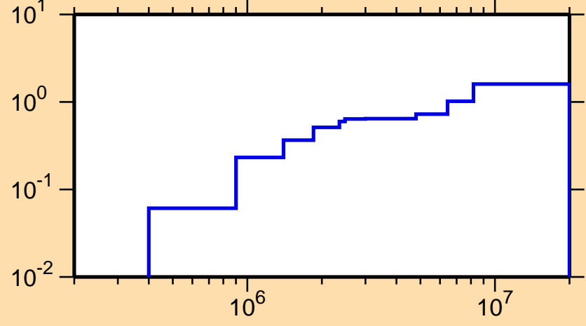
\sigma vs. E for ^{201}\text{Rn}(n,\text{inel.})
