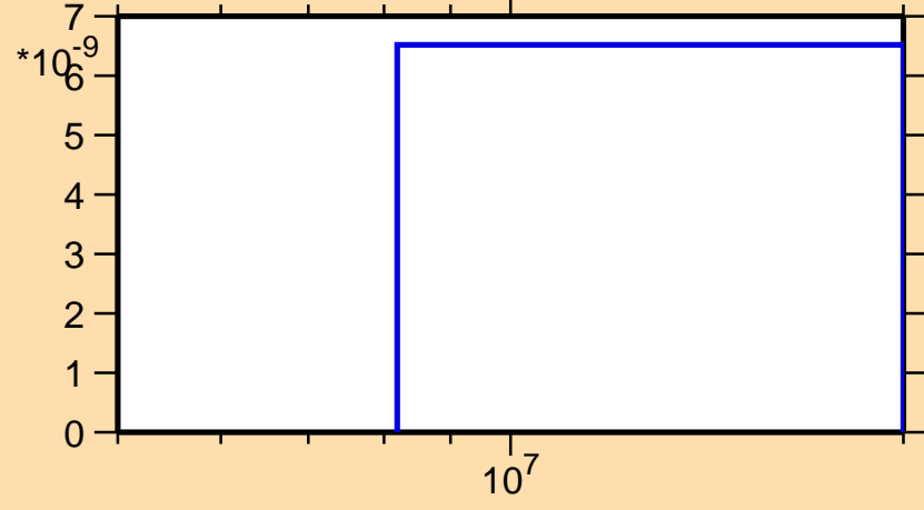
\sigma vs. E for ^{201}\text{Rn}(n,\text{pd})
