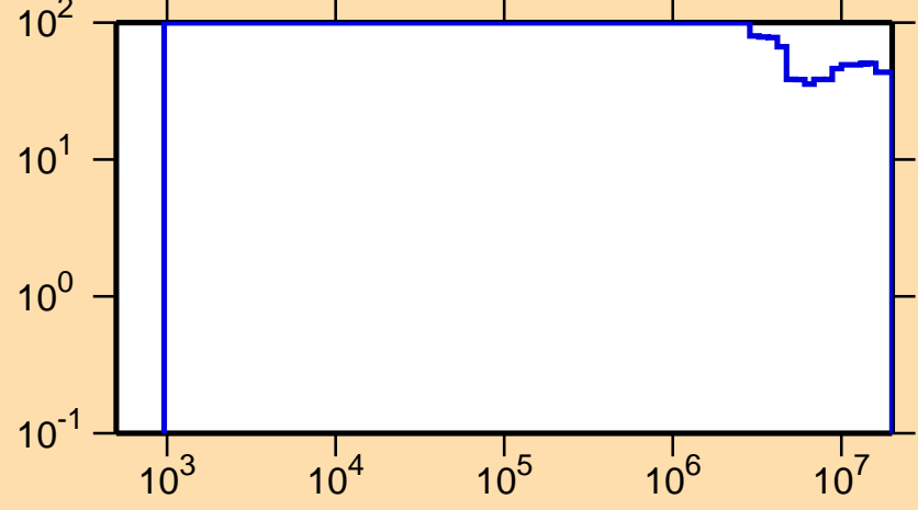
\Delta\sigma/\sigma vs. E for ^{201}\text{Rn}(n,n\text{cont.})
