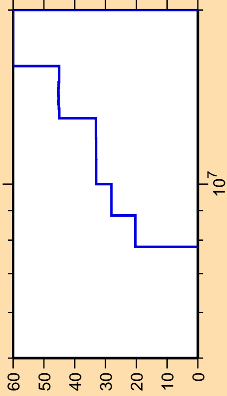
\Delta\sigma/\sigma vs. E for ^{201}\text{Rn}(n,\gamma)
