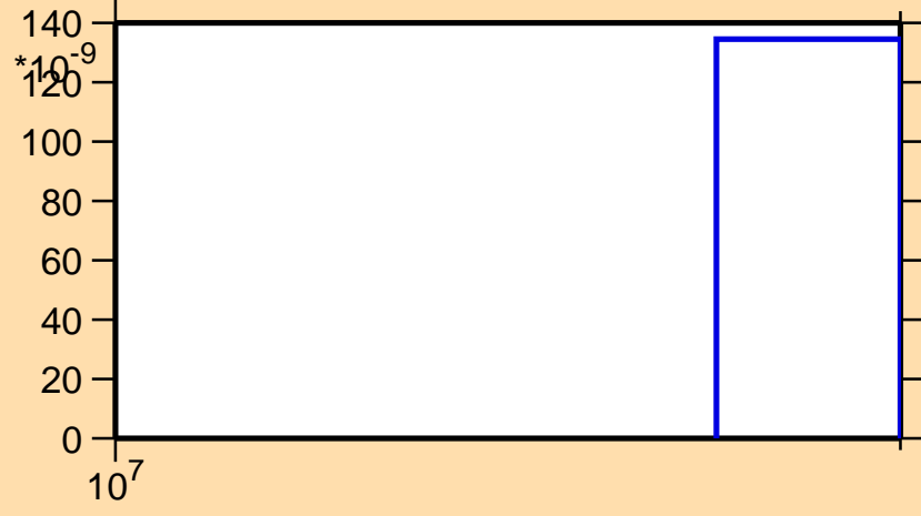
\sigma vs. E for ^{201}\text{Rn}(n,3n)
