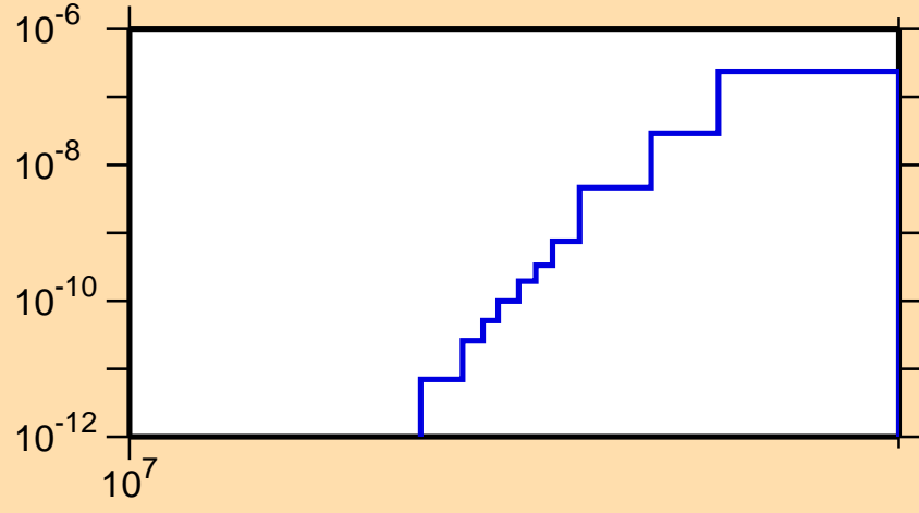
\sigma vs. E for ^{201}\text{Rn}(n,\text{nd})
