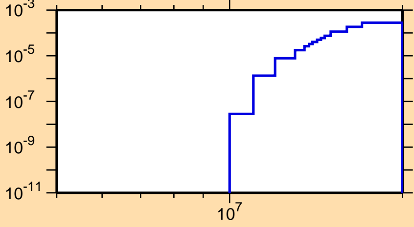
\sigma vs. E for ^{201}\text{Rn}(n,2n\alpha)
