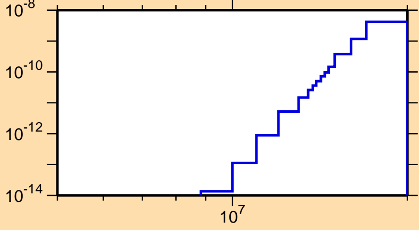
\sigma vs. E for ^{201}\text{Rn}(\text{mt117})
