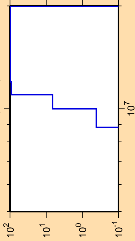
\Delta\sigma/\sigma vs. E for ^{201}\text{Rn} (mt 45)
