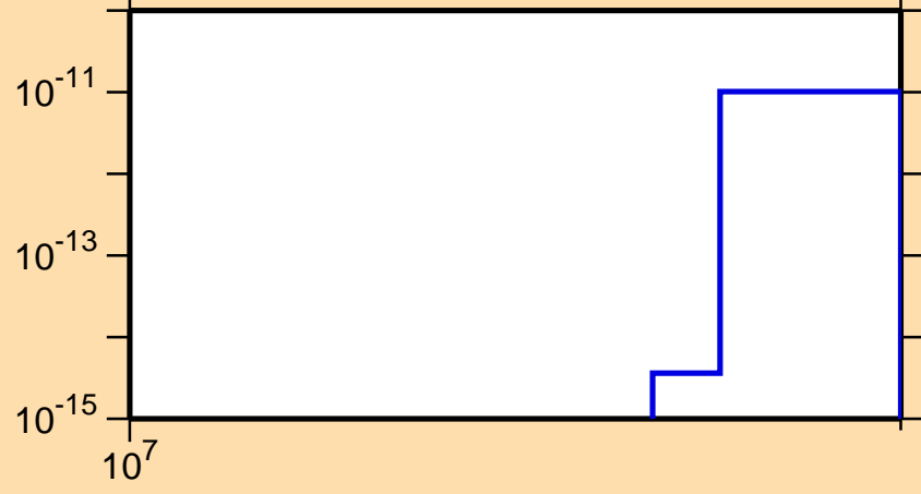
\sigma vs. E for ^{201}\text{Rn}(n,nt)
