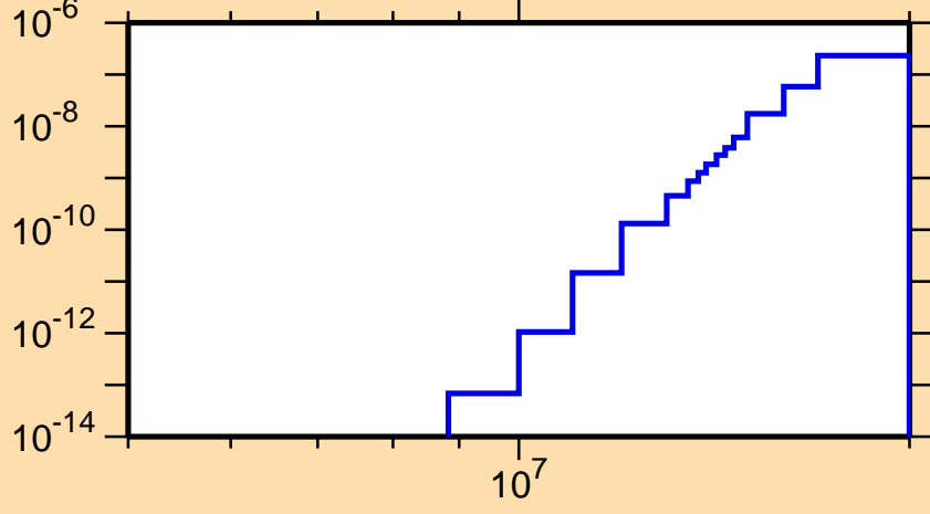
\sigma vs. E for ^{201}\text{Rn} (mt 45)
