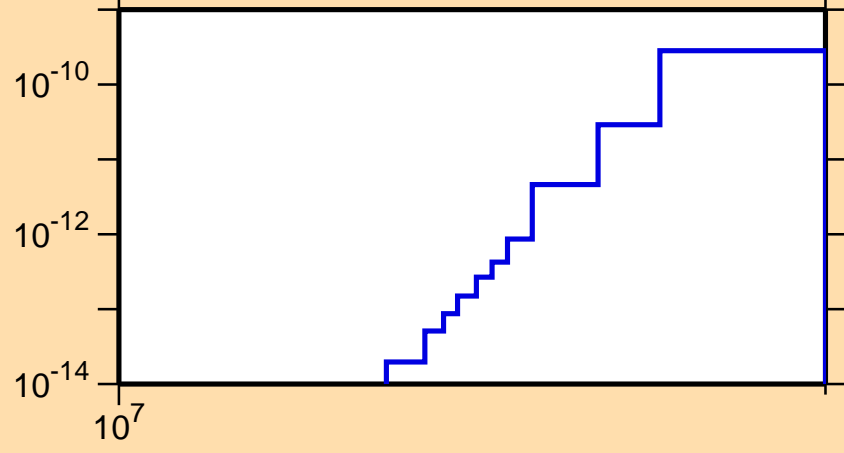
\sigma vs. E for ^{201}\text{Rn} (mt 34)
