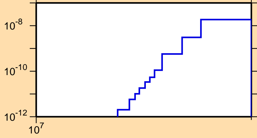
\sigma vs. E for ^{201}\text{Rn}(n,\text{pt})
