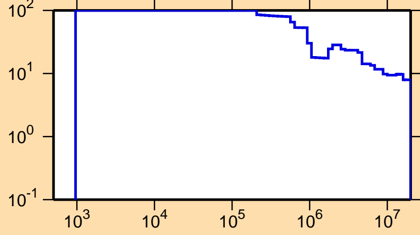
\Delta\sigma/\sigma vs. E for ^{201}\text{Rn}(n,\text{nonel.})
