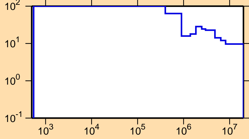
\Delta\sigma/\sigma vs. E for ^{201}\text{Rn}(n,n\text{onel.})
