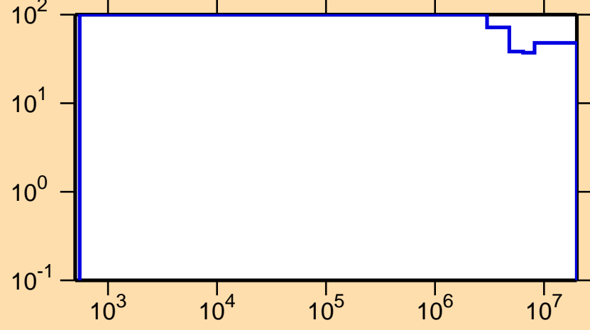
\Delta\sigma/\sigma vs. E for ^{201}\text{Rn}(n,ncont.)
