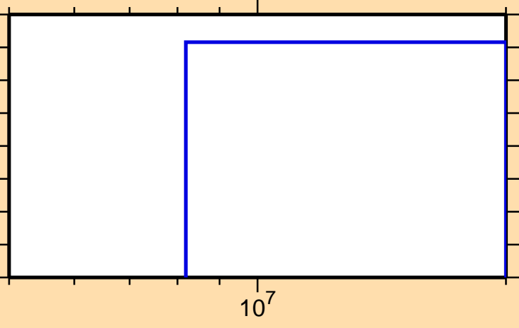
\sigma vs. E for ^{201}\text{Rn}(n,3n\alpha)
