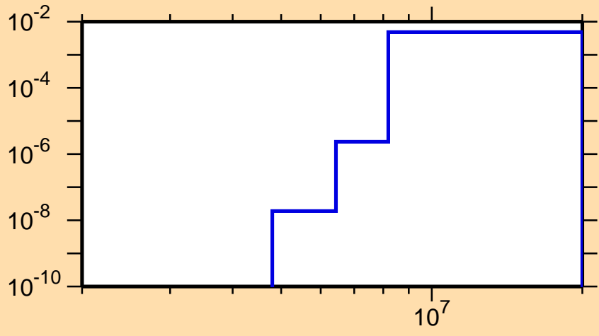
\sigma vs. E for ^{201}\text{Rn}(n,d)
