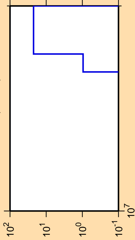
\Delta\sigma/\sigma vs. E for ^{202}\text{Rn} (mt 34)
