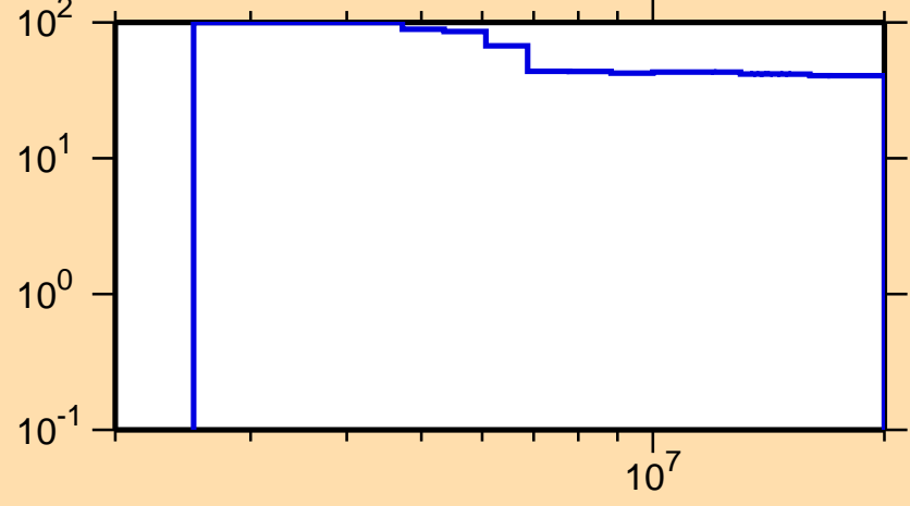
\Delta\sigma/\sigma vs. E for ^{202}\text{Rn}(n,n\text{cont.})
