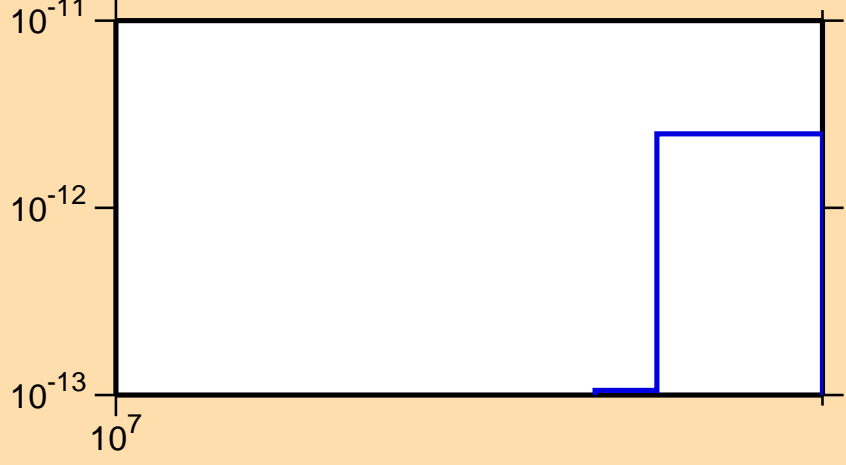
\sigma vs. E for ^{202}\text{Rn} (mt 34)
