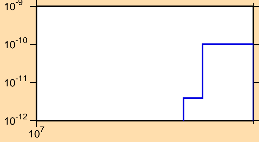
\sigma vs. E for ^{202}\text{Rn}(n,pt)
