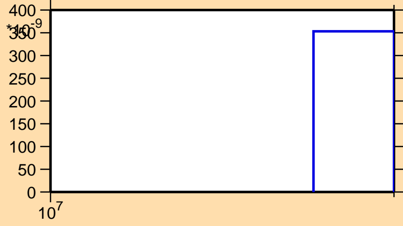
\sigma vs. E for ^{202}\text{Rn}(n,3n)
