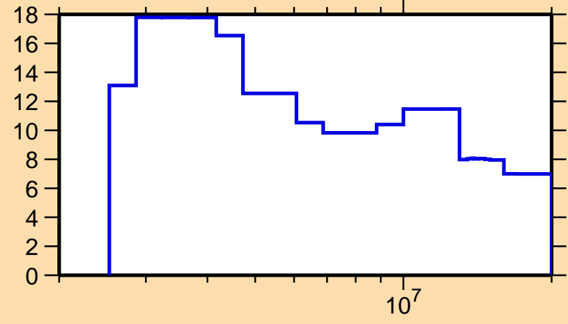
\Delta\sigma/\sigma vs. E for ^{202}\text{Rn}(n,\text{tot.})
