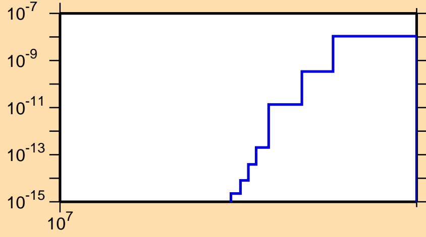
\sigma vs. E for ^{202}\text{Rn}(n,nd)
