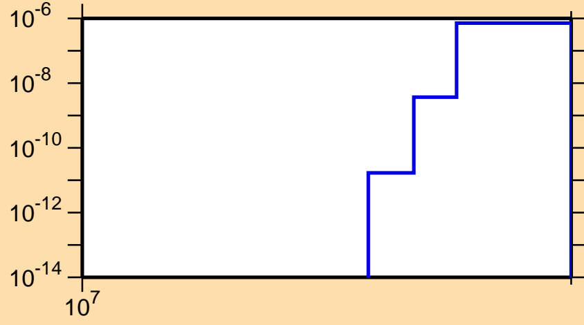
\sigma vs. E for ^{202}\text{Rn}(n,2np)
