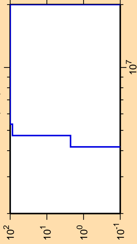
\Delta\sigma/\sigma vs. E for ^{202}\text{Rn}(n,d)
