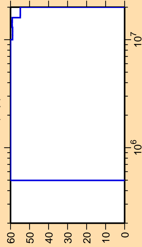
\Delta\sigma/\sigma vs. E for ^{202}\text{Rn}(n,p)
