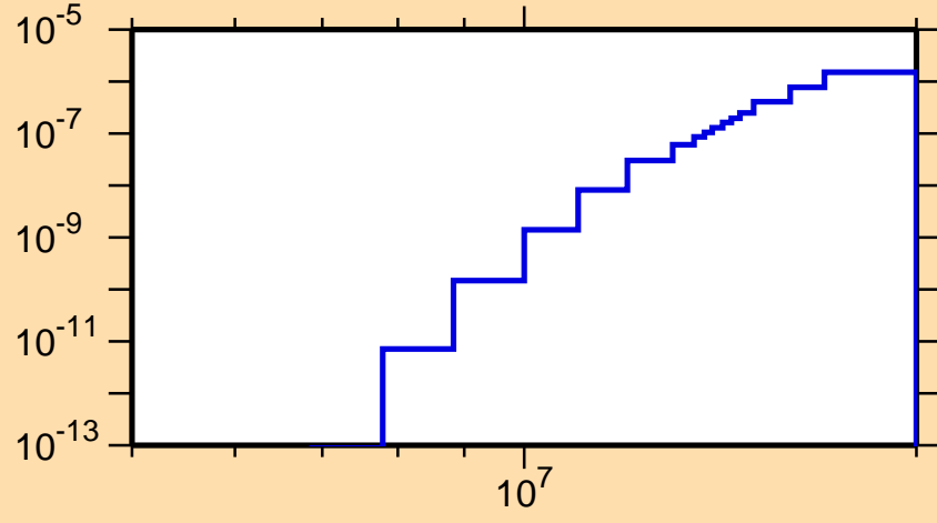
\sigma vs. E for ^{202}\text{Rn}(\text{mt } 45)
