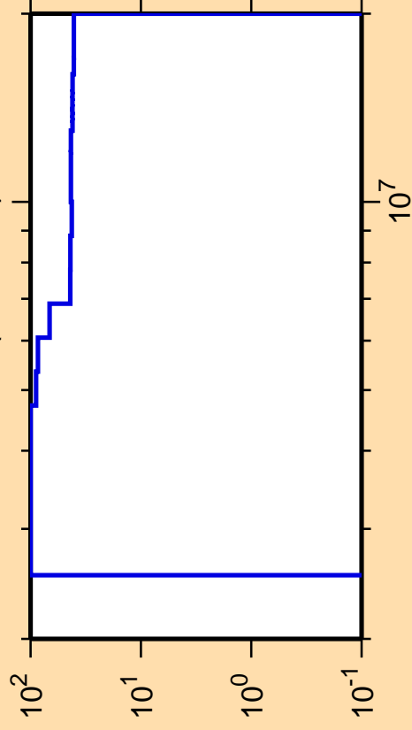
\Delta\sigma/\sigma vs. E for ^{202}\text{Rn}(n,n\text{cont.})
