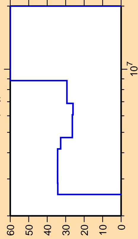
\Delta\sigma/\sigma vs. E for ^{202}\text{Rn}(n,\gamma)
