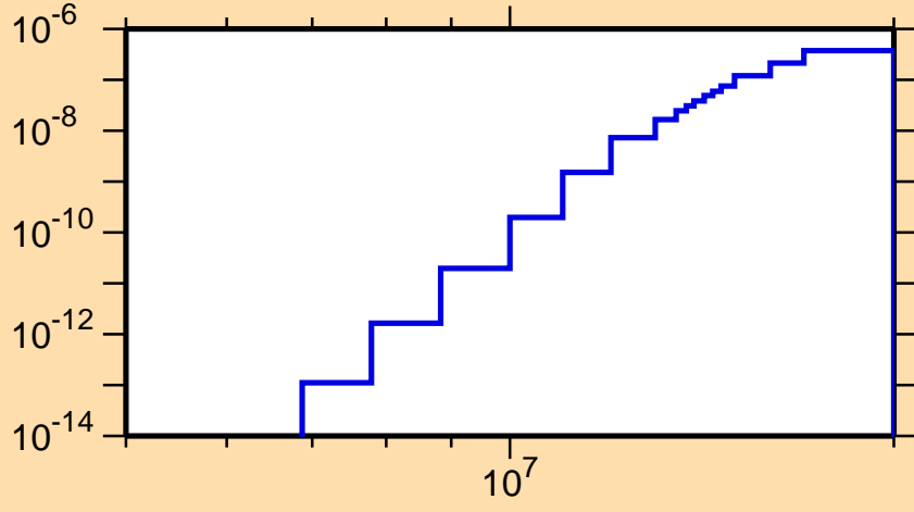
\sigma vs. E for ^{202}\text{Rn}(\text{mt117})
