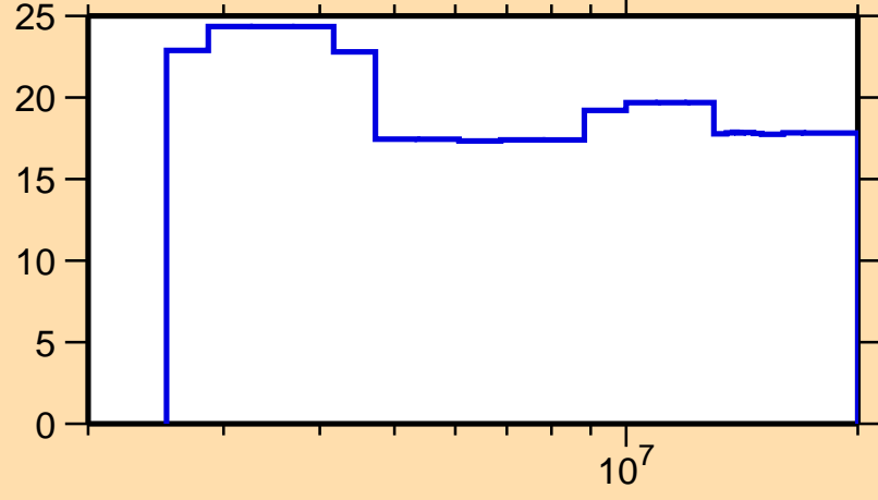
\Delta\sigma/\sigma vs. E for ^{202}\text{Rn}(n,\text{nonel.})
