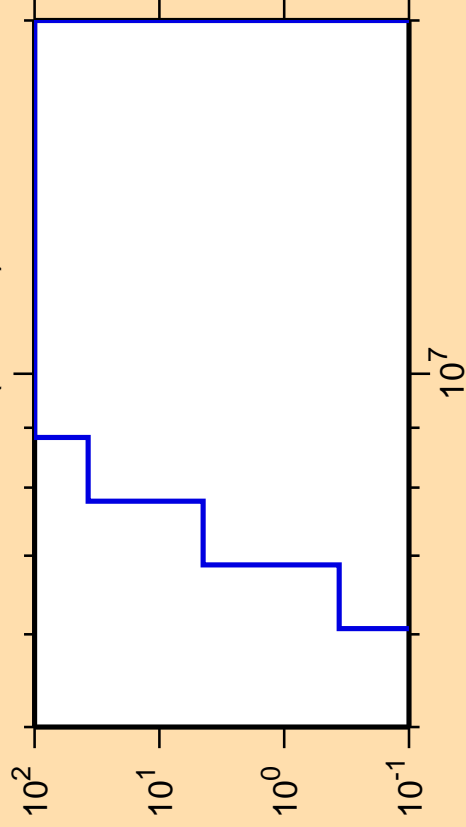
\Delta\sigma/\sigma vs. E for ^{202}\text{Rn}(n,\text{He}3)
