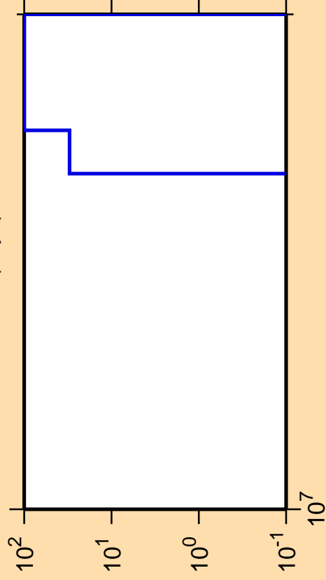
\Delta\sigma/\sigma vs. E for ^{202}\text{Rn}(n,pt)
