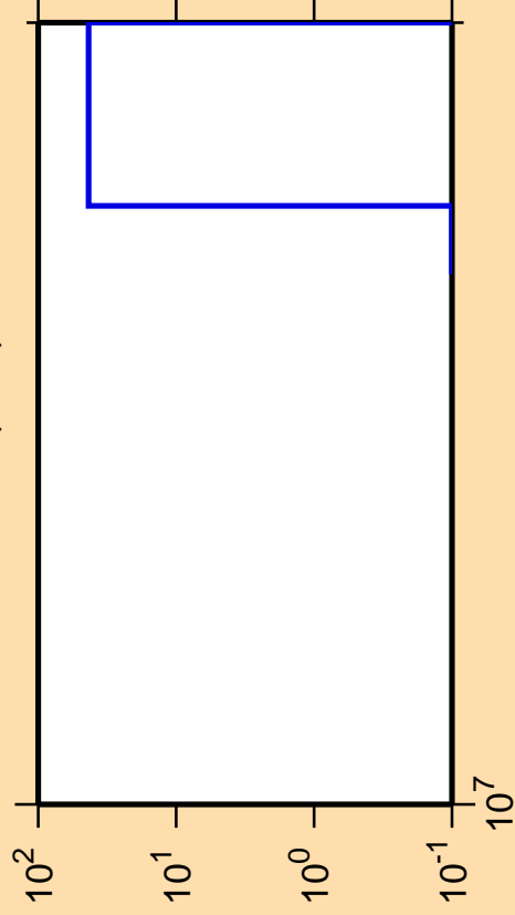
\Delta\sigma/\sigma vs. E for ^{202}\text{Rn}(n,nt)
