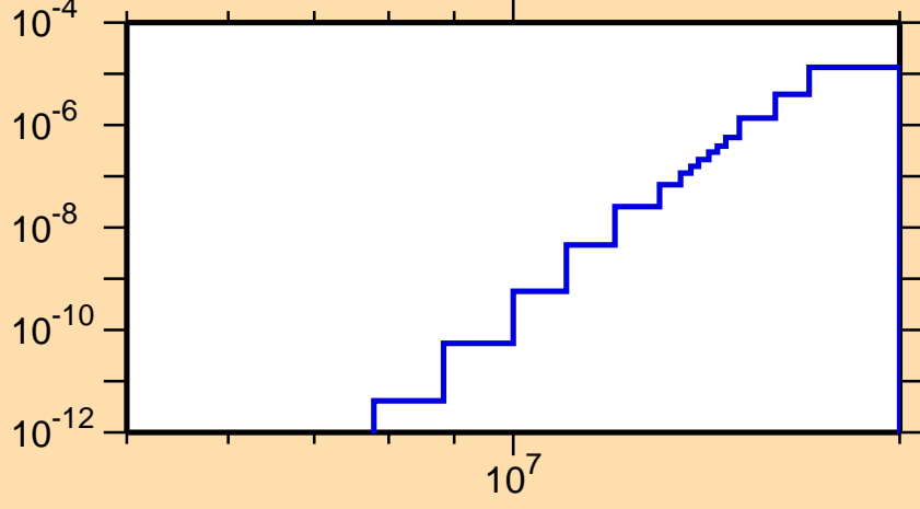
\sigma vs. E for ^{202}\text{Rn}(n,\text{He}3)
