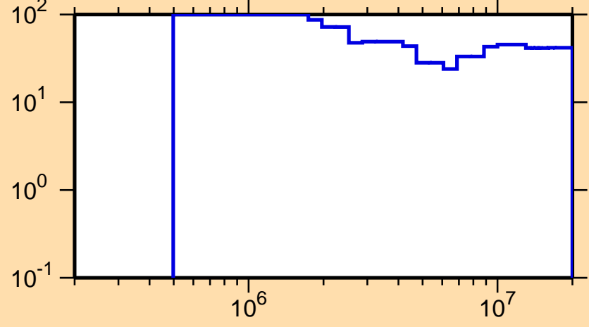
\Delta\sigma/\sigma vs. E for ^{202}\text{Rn}(n,\text{inel.})
