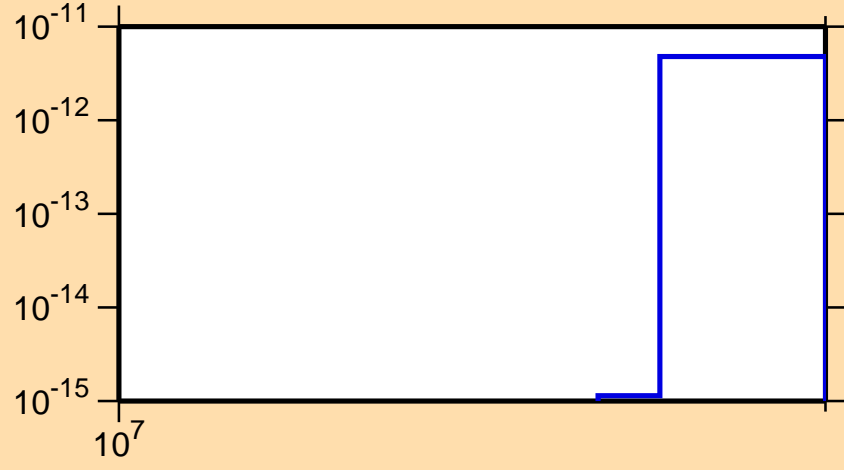
\sigma vs. E for ^{202}\text{Rn}(n,nt)
