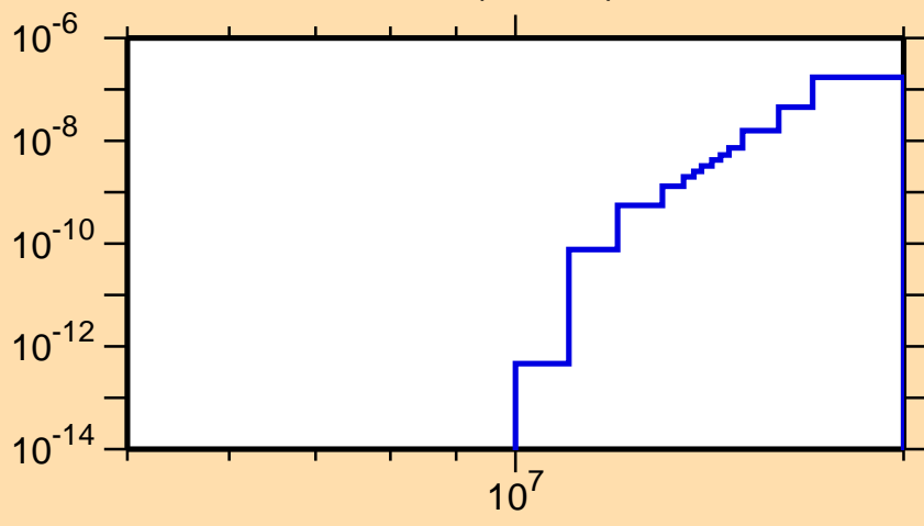
\sigma vs. E for ^{202}\text{Rn}(n,2n\alpha)
