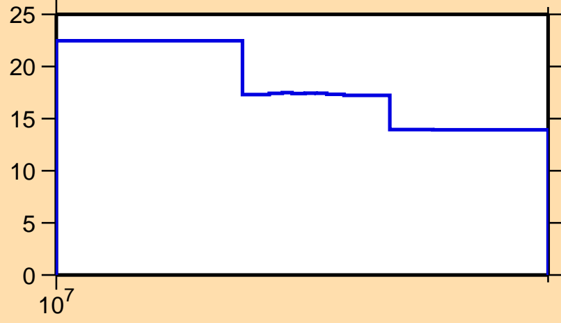
\Delta\sigma/\sigma vs. E for ^{202}\text{Rn}(n,\text{el.})
