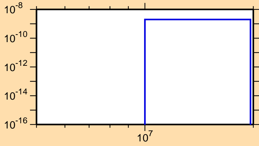
\sigma vs. E for ^{202}\text{Rn}(n,\text{pd})
