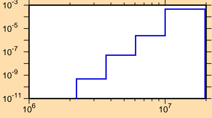
\sigma vs. E for ^{202}\text{Rn}(n,n\alpha)
