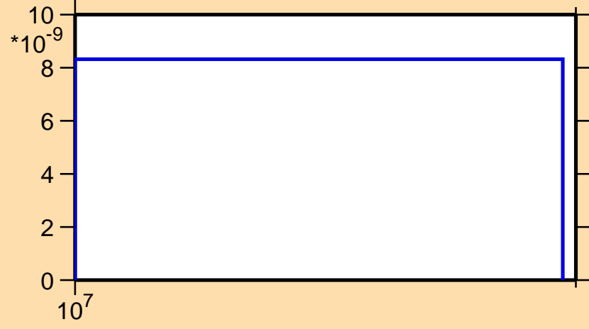
\sigma vs. E for ^{202}\text{Rn}(n,2n\alpha)
