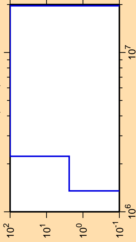
\Delta\sigma/\sigma vs. E for ^{202}\text{Rn}(n,n\alpha)
