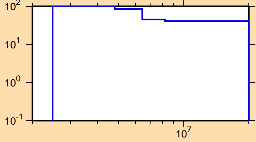
\Delta\sigma/\sigma vs. E for ^{202}\text{Rn}(n,ncont.)
