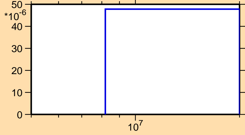
\sigma vs. E for ^{202}\text{Rn}(n,t)
