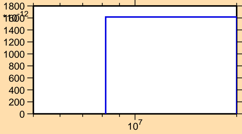
\sigma vs. E for ^{202}\text{Rn}(n,\text{pd})
