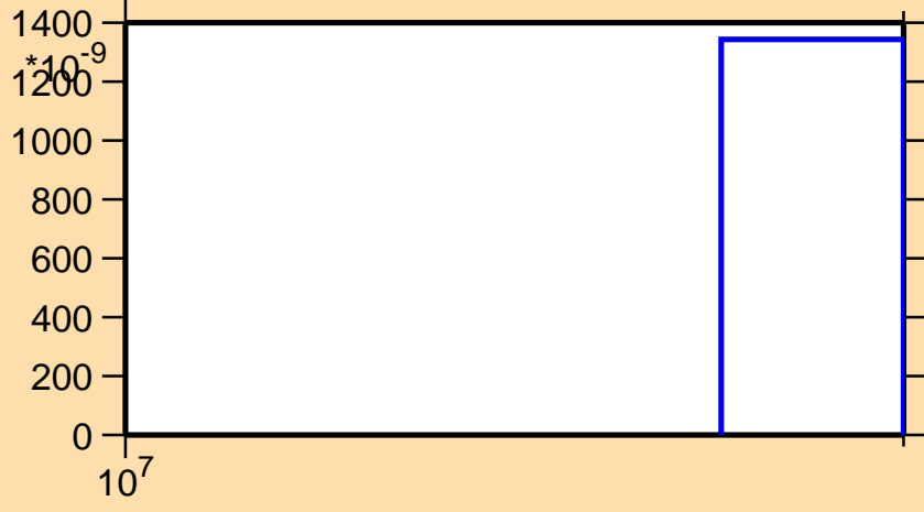
\sigma vs. E for ^{203}\text{Rn}(n,3n)
