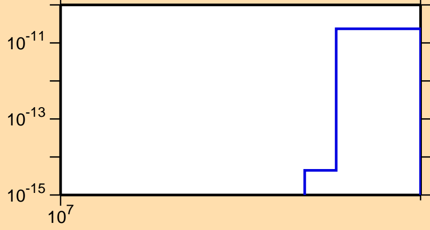
\sigma vs. E for ^{203}\text{Rn}(n,nt)
