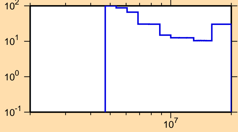
\Delta\sigma/\sigma vs. E for ^{203}\text{Rn}(n,ncont.)
