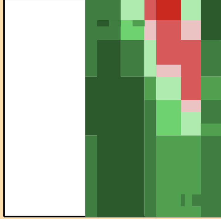
\Delta\sigma/\sigma vs. E for ^{203}\text{Rn}(n,n\text{cont.})
