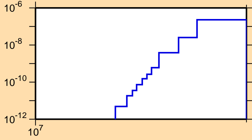
\sigma vs. E for ^{203}\text{Rn}(n,\text{nd})
