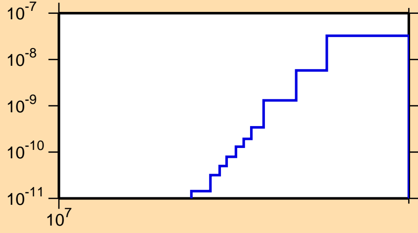
\sigma vs. E for ^{203}\text{Rn} (mt 45)
