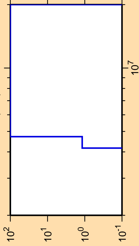
\Delta\sigma/\sigma vs. E for ^{203}\text{Rn}(n,d)
