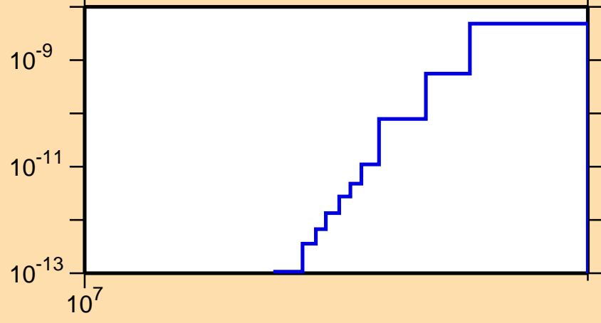
\sigma vs. E for ^{203}\text{Rn}(n,\text{pt})
