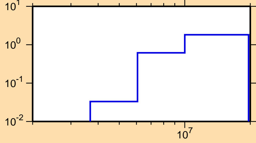
\sigma vs. E for ^{203}\text{Rn}(n,n\text{cont.})
