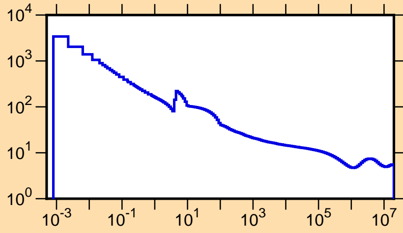
\sigma vs. E for ^{203}\text{Rn}(n,\text{tot.})
