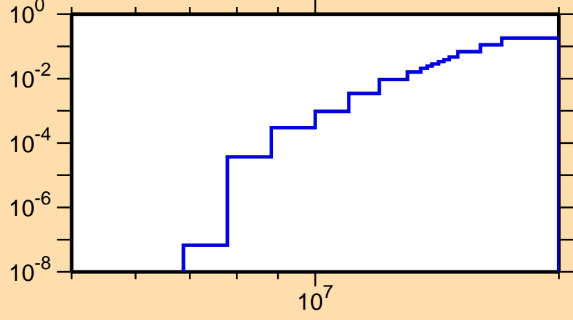
\sigma vs. E for ^{203}\text{Rn}(n,2n)
