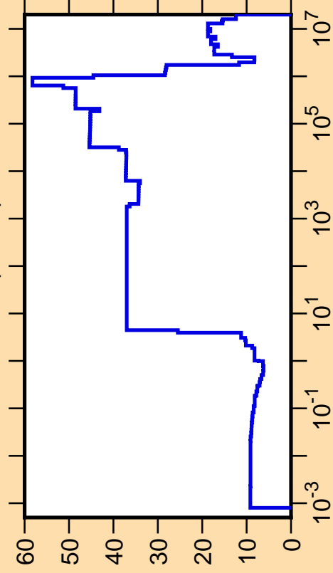
\Delta\sigma/\sigma vs. E for ^{203}\text{Rn}(n,\text{tot.})
